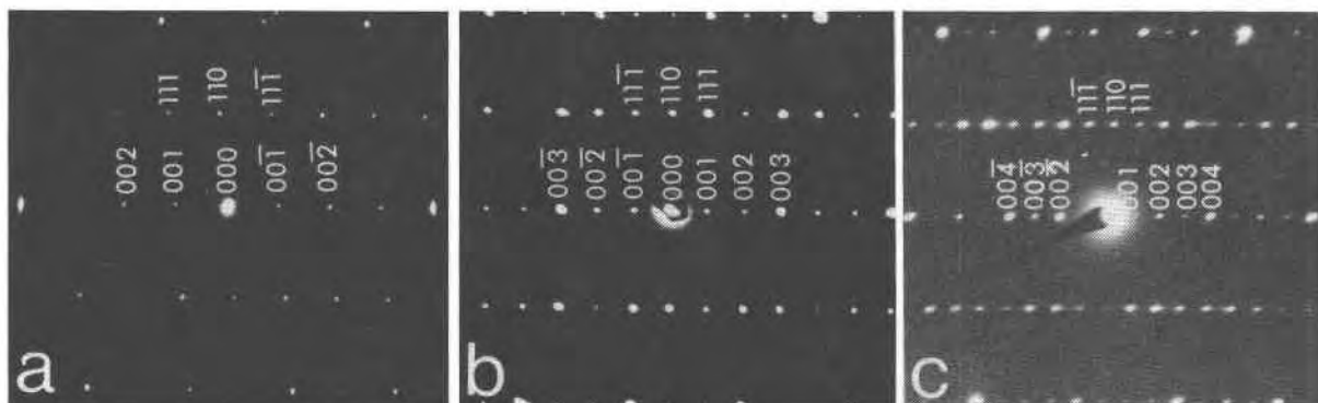
Fig. 14. Diffraction patterns of three (r)^n structures recorded in the [110]_c zone: (a) (d-d) aristotype ( \text{CaZrTi}_2\text{O}_7 ); (b) (t)^3 hettotype ( \text{Ca}_{0.77}\text{Th}_{0.24}\text{ZrTi}_{1.5}\text{Al}_{0.5}\text{O}_7 ); (c) (r)^4 hettotype ( \text{Ca}_{0.5}\text{SmZr}_{0.5}\text{Ti}_2\text{O}_7 ).
