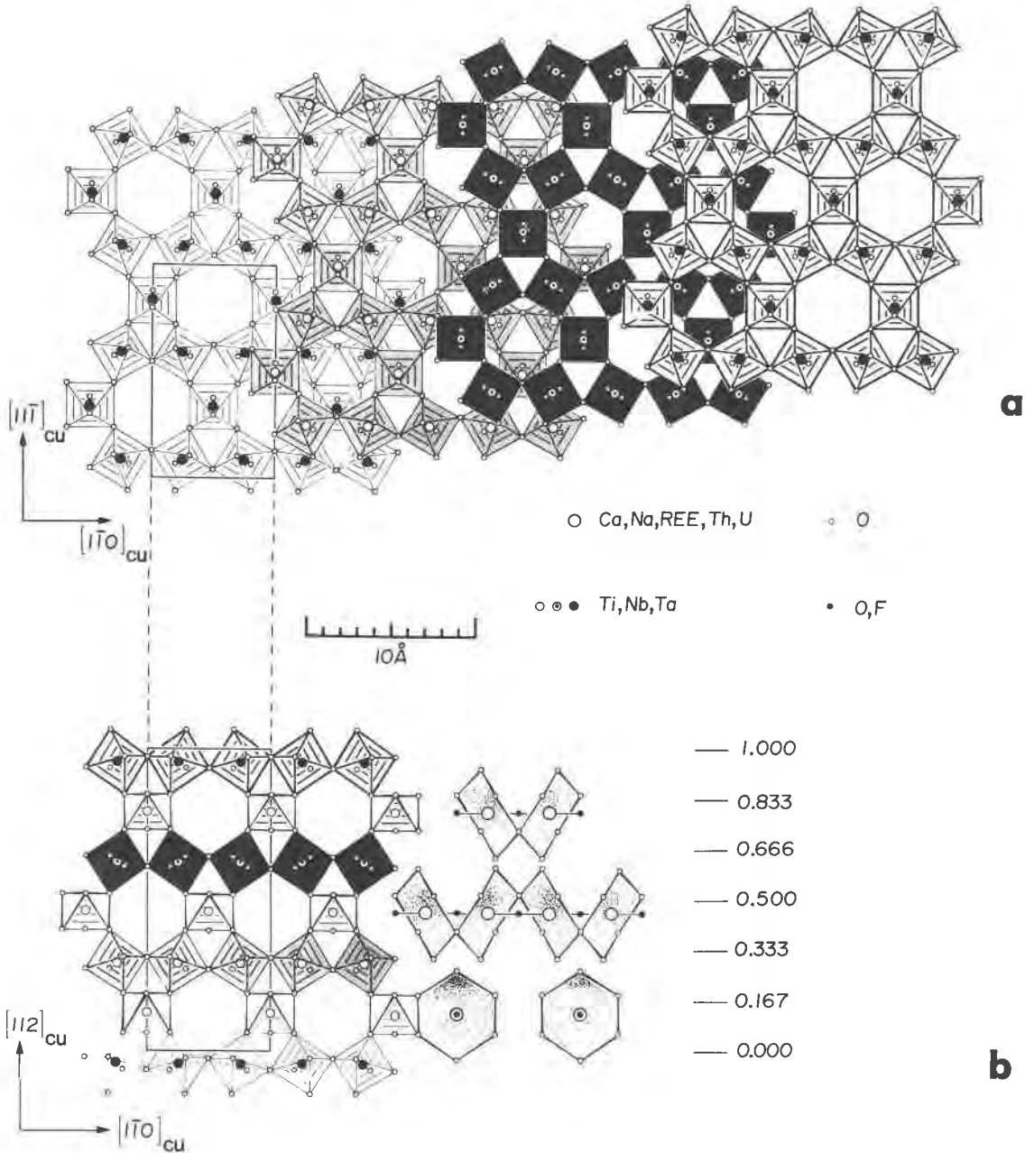
Fig. 5. (a) The pyrochlore structure projected down [001]_c = [110]_{cu} emphasizing the HTB layers. (b) The [100]_c = [111]_{cu} projection. HTB layers occur at z = 0.292, 0.625 and 0.958 . (c) An interlayer region containing A ( O_6F_2 ) puckered hexagonal bipyramids and BO_6 octahedra. On the right the correspondence between the bipyramid and a distorted cube is shown (Mazzi and Munno, 1983).
