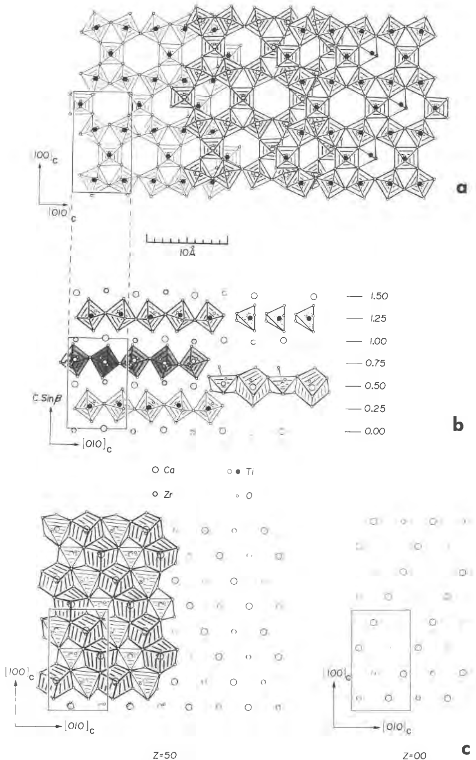
Fig. 3. (a) The zirconolite structure projected down c^* . \text{TiO}_6 octahedra are arranged in an HTB type motif; the unshaded layers on the extreme left and right are equivalent and correspond to the lower most and uppermost layers respectively. The stippled polyhedra in the six-membered octahedral rings represent one of a statistical pair of \text{TiO}_5 trigonal bipyramids. (b) The [100]_c projection. On the left \text{TiO}_6 octahedra at z = \pm 0.25 are emphasized; on the right some of the distorted \text{CaO}_8 cubes, \text{ZrO}_7 face-capped octahedra and \text{TiO}_5 trigonal bipyramids are shown. (c) The polyhedra of the interlayer cation planes. Strings of \text{CaO}_8 cubes alternate with chains of \text{ZrO}_7 face-capped octahedra. These run parallel to [\bar{1}10]_c and [110]_c at z = 50 and z = 0 respectively. (Gatehouse et al., 1981).
