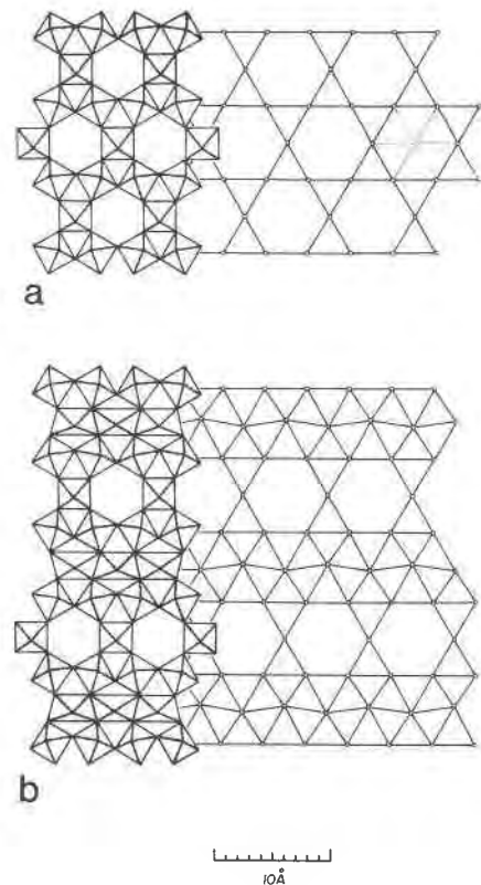
Fig. 7. (a) The cation nodes of an HTB array correspond to a kagomé net. If the cation site at the center of the six-membered ring were occupied a triangular net would result (dotted lines). (b) In polymignyte the cation nodes of the modified HTB layer yield a net which is an intergrowth between the kagomé net and a distorted triangular net.
