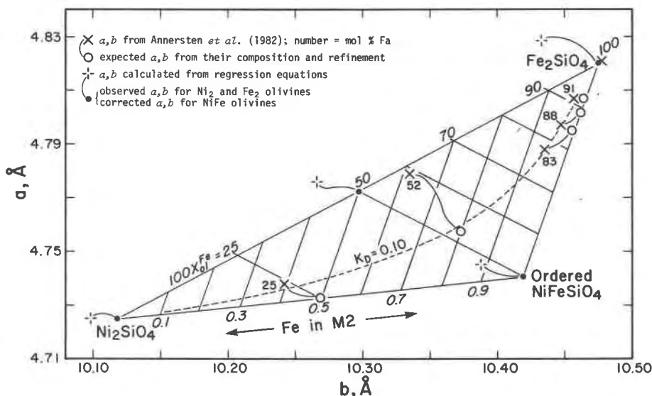
Fig. 1. An a - b plot for Fe-Ni olivines. Values for the end-members, \text{Ni}_2\text{SiO}_4 and \text{Fe}_2\text{SiO}_4 , respectively, are averages of 4 and 5 sets of cell dimensions taken from the literature. Other data are from Table 1; details of construction and interpretation are in the text. The dashed curve is a line of constant K_D = 0.10 .
