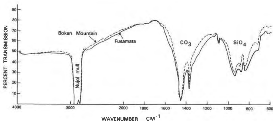
Fig. 1. Infrared transmission spectra for iimoriite from Bokan Mountain, Alaska and Fusamata, Japan.
