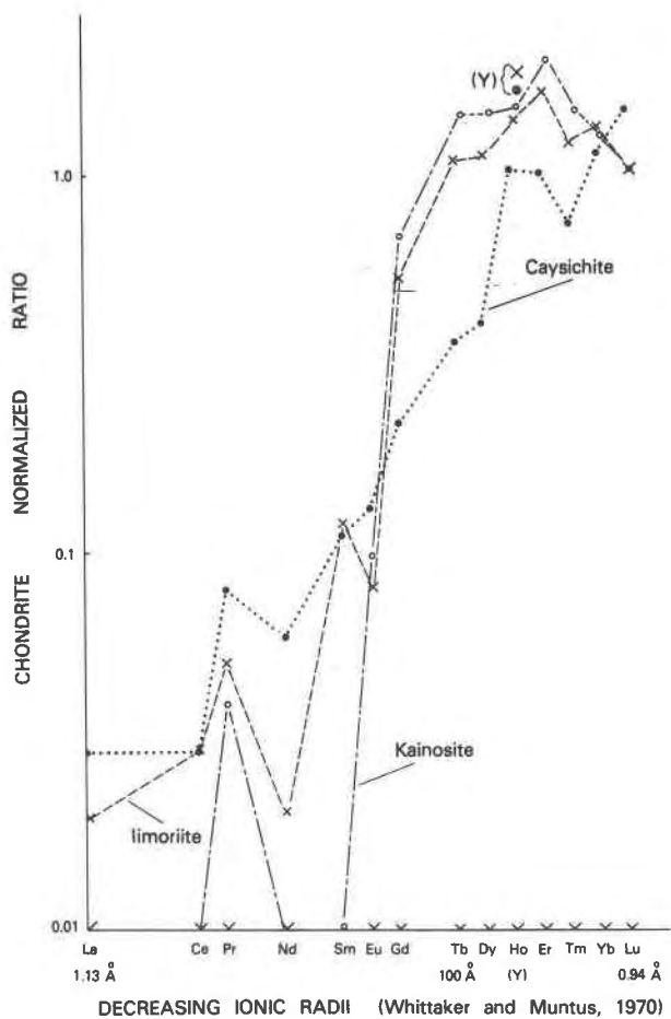
Fig. 2. Chondrite normalized ratios for iimoriite, caysichite, and kainosite.
