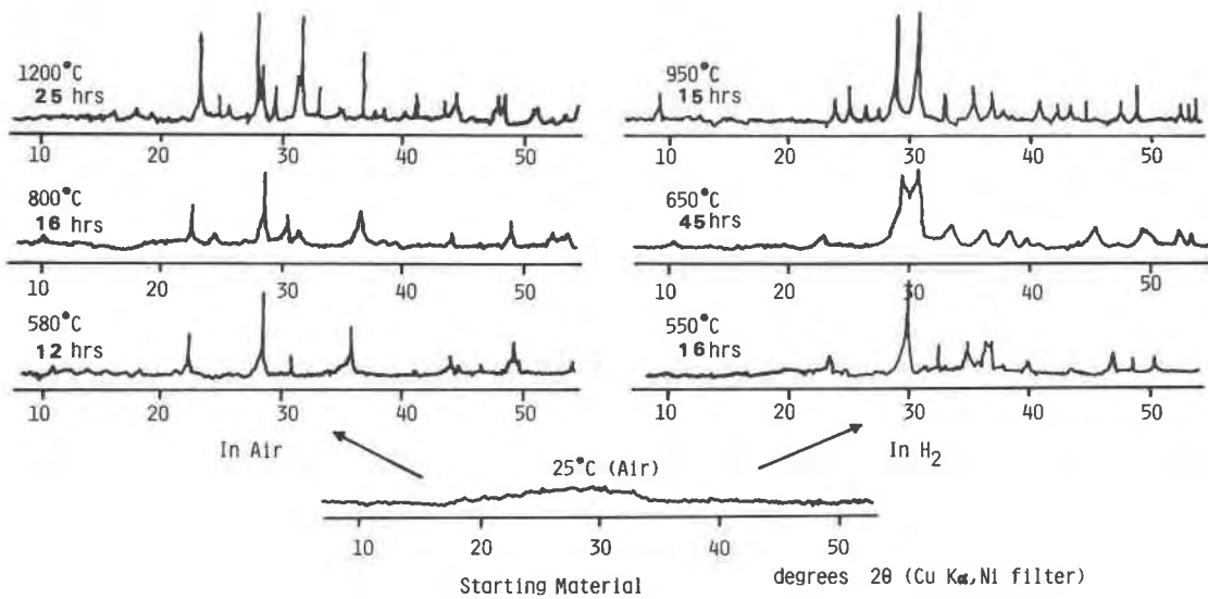
Fig. 1. X-ray powder patterns of samarskite, Kawabe, Fukushima Prefecture, Japan, heated in oxidizing and in reducing atmospheres. Heating time and temperature are indicated on the diffractograms.
