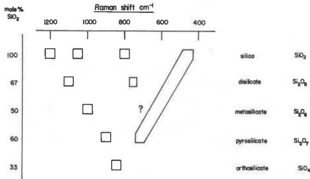
Fig. 1. Schematic of major band groups maximized as a function of silica content in alkali and alkaline earth glass and melt series. The low-frequency ( 700\text{--}400\text{ cm}^{-1} ) group is shown here as a single continuously varying band. In fact, discrete bands are observed in this region (see text), but their behavior with composition is not yet well characterized.
