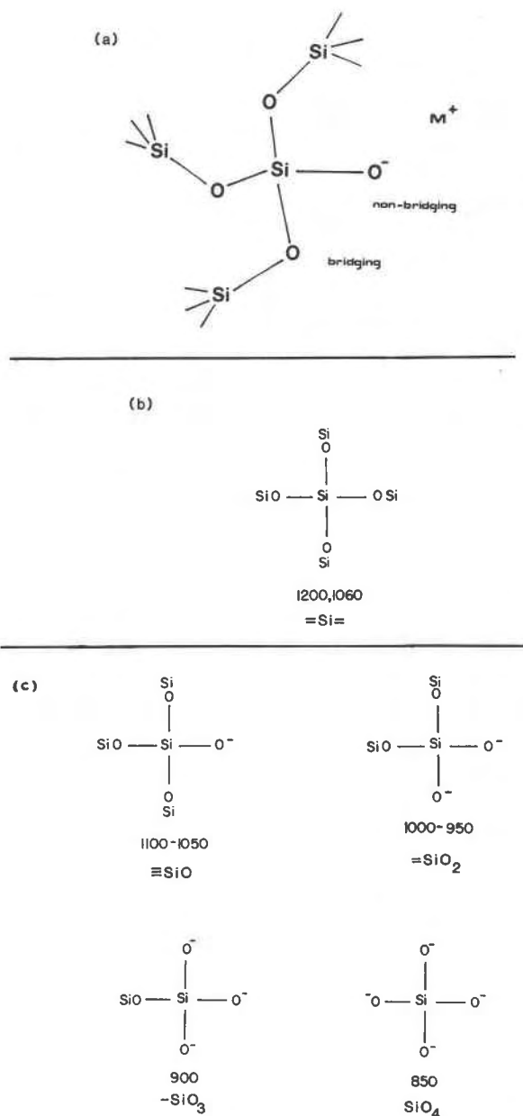
Fig. 2. Silicate structural units. (a) Schematic indicating the nature of bridging and non-bridging oxygen in the present context. M^+ may also refer to 0.5 M^{2+} , as in the alkaline earth series; (b) The weak, depolarized bands at 1200 and 1060\text{ cm}^{-1} are thought to correspond to asymmetric silicon-oxygen stretching vibrations within a fully-polymerized tetrahedral network =\text{Si}=\text{O} ; (c) The four major polarized high-frequency bands are generally assigned to symmetric stretching vibrations of tetrahedral silicate units with one, two, three and four non-bridging oxygens.
