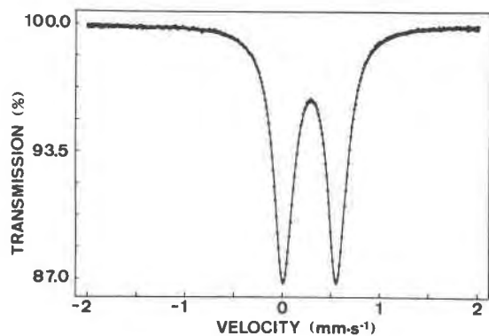
Fig. 1. Mössbauer spectrum of paramagnetic andradite at 121(2) K.
