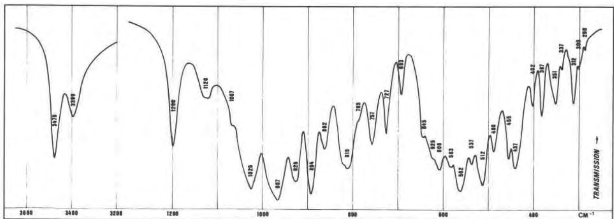
Fig. 1. Infrared spectrum of davreuxite from Otrré.
