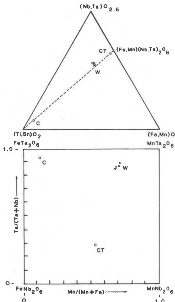
Fig. 2. The Herbb #2 minerals in the (\text{Nb,Ta})\text{O}_{2.5} – (\text{Fe,Mn})\text{O} – (\text{Ti,Sn})\text{O}_2 triangle and in the columbite–tantallite quadrilateral (W—wodginite, CT—manganocolumbite, C—cassiterite).
