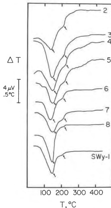
Fig. 3. Representative DTA patterns at 1 atmosphere of SWy-1 and each size fraction from #2 to #8 (see Table 1). Arrows correspond to points (c) and (e) in Fig. 2 and represent two stages of dehydration. The peaks and their locations were verified by duplicate runs. Note that particle size is not a major influence in defining the dehydration temperature, but fraction #8 does show the sharpest peak and the weakest shoulder.
