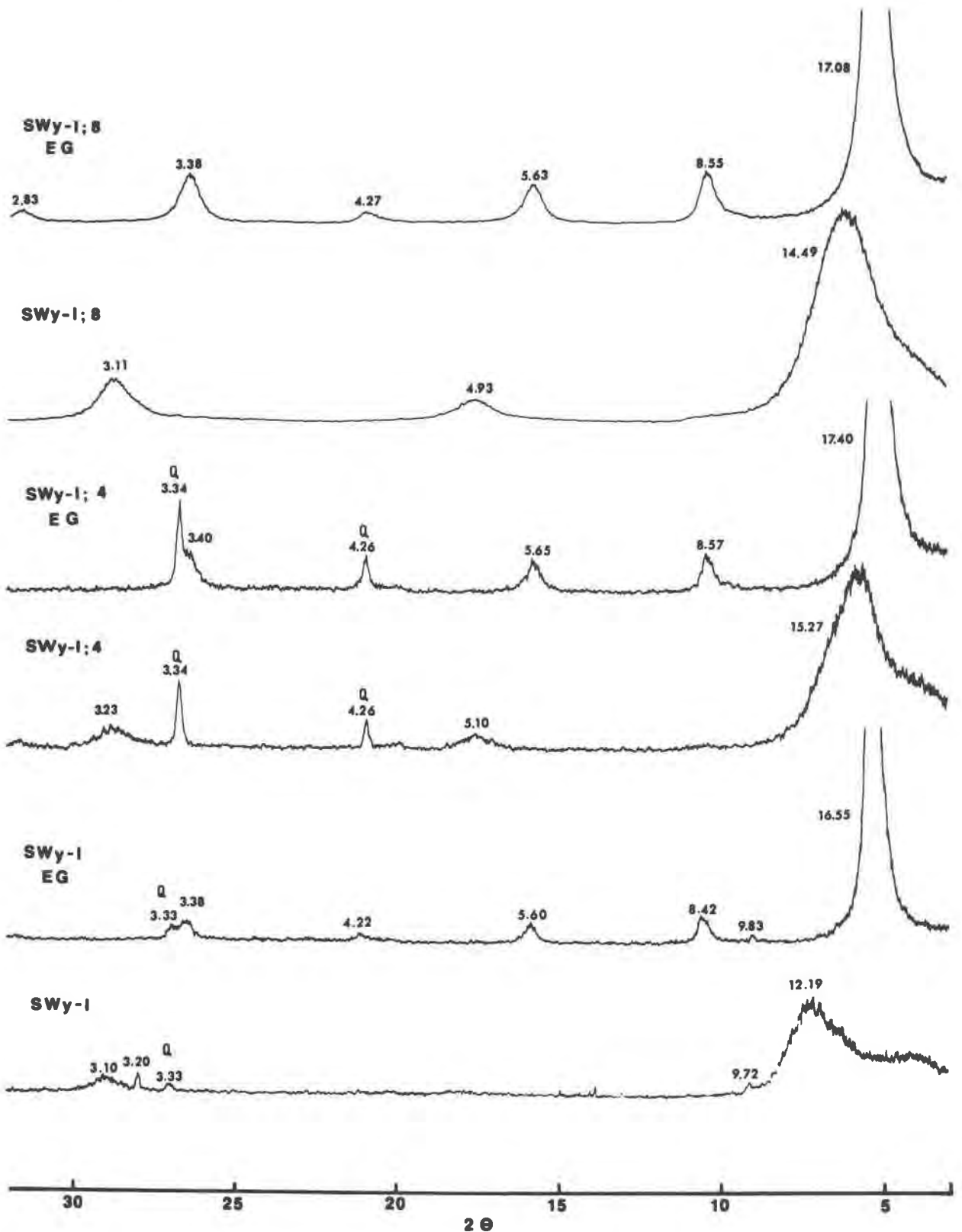
Fig. 1. X-ray diffractograms (CuK \alpha radiation, Ni-filtered, 1°/min) of SWy-1 as received and of size fraction #4 and 8 (see Table I) at 55% relative humidity and glycolated (EG).
