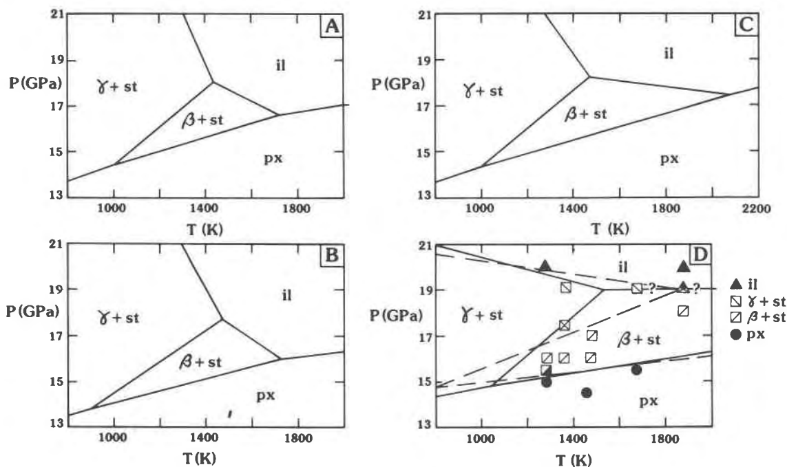
Fig. 1. Calculated MgSiO_3 phase relations. Fig. 1A, B, C represents calculations based on thermochemical data sets A, B, C in Table 3, respectively. Fig. 1D shows the experimental synthesis data of E. Ito (1984, unpublished). See text for discussion of boundaries.
