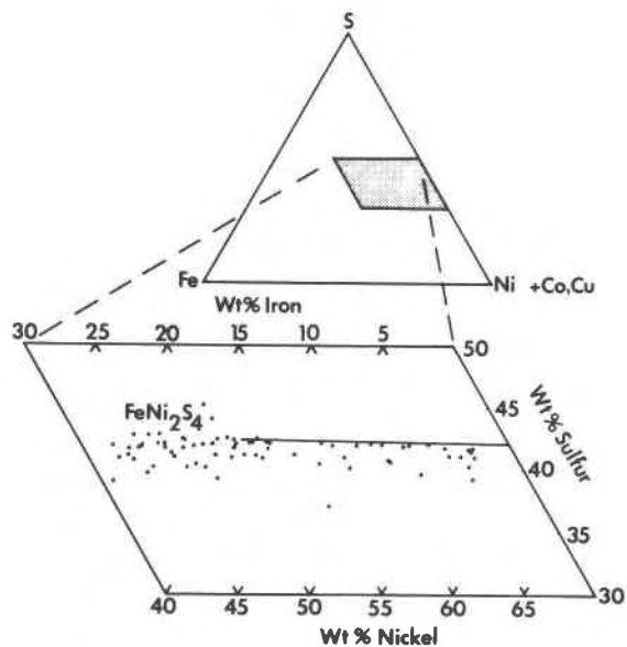
Fig. 8. Compositions of natural iron-nickel thiospinels shown in terms of Fe, Ni and S content (for sources of data, see Table 2).
