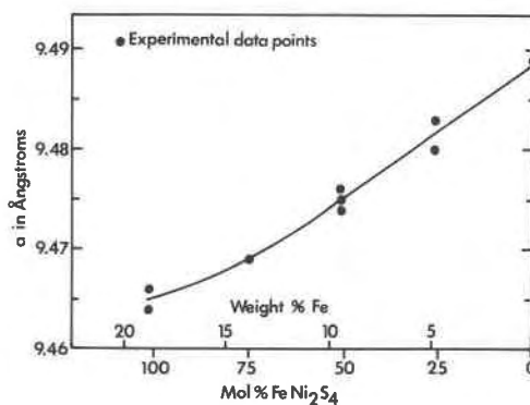
Fig. 2. Variation in unit cell parameter ( a ) with composition between \text{FeNi}_2\text{S}_4 and \text{Ni}_3\text{S}_4 . The unit cell parameter of \text{Fe}_3\text{S}_4 is 9.876 Å.
