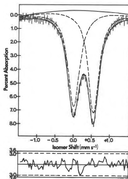
Fig. 5. Computer fit of a simple doublet to the Mössbauer spectrum of FeNi _2 S _4 .
