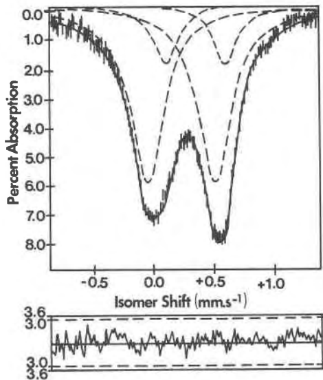
Fig. 6. Computer fit of two doublets to the Mössbauer spectrum of \text{FeNi}_2\text{S}_4 .
