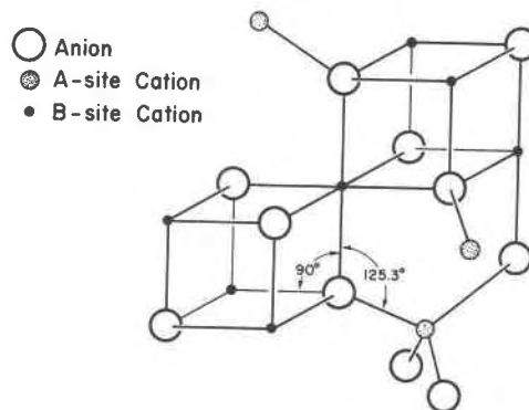
Fig. 1. The spinel crystal structure showing the relationships between cations in octahedral and tetrahedral coordination.
