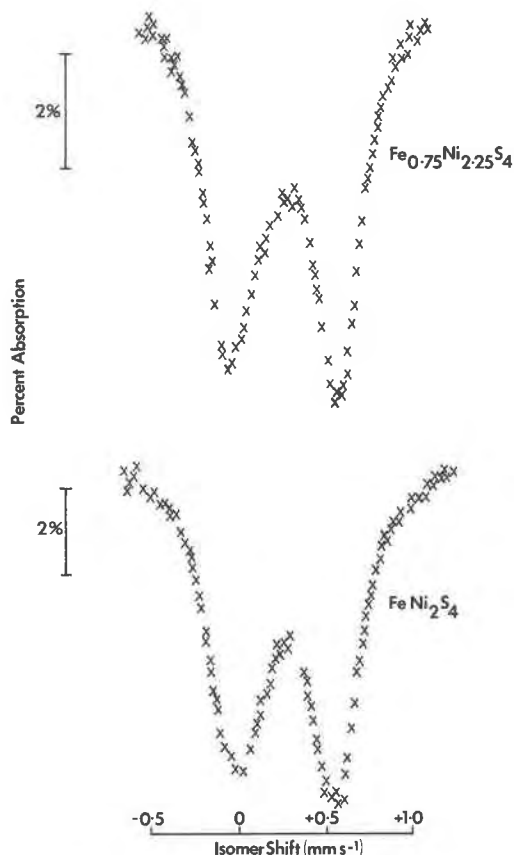
Fig. 4. Mössbauer spectra for violarites of varying iron content; the zero of the velocity scale is the center of gravity of an iron foil spectrum.
