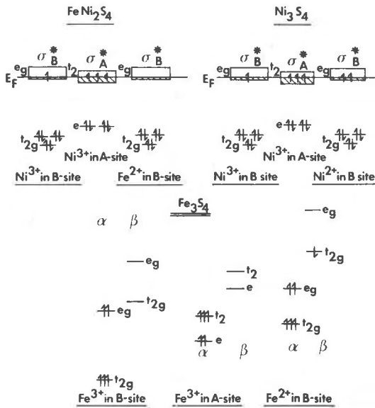
Fig. 9. Schematic energy level diagrams for the 3d orbitals in \text{Ni}_3\text{S}_4 , \text{FeNi}_2\text{S}_4 and \text{Fe}_3\text{S}_4 . \alpha and \beta refer to spin directions of the electrons; E_F is the Fermi level.
