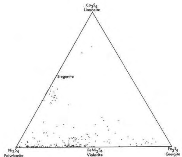
Fig. 7. Compositions of natural iron-nickel thiospinels shown in terms of \text{Fe}_3\text{S}_4 – \text{Ni}_3\text{S}_4 – \text{Co}_3\text{S}_4 endmembers to illustrate the variation in cation contents (for sources of data see Table 2).
