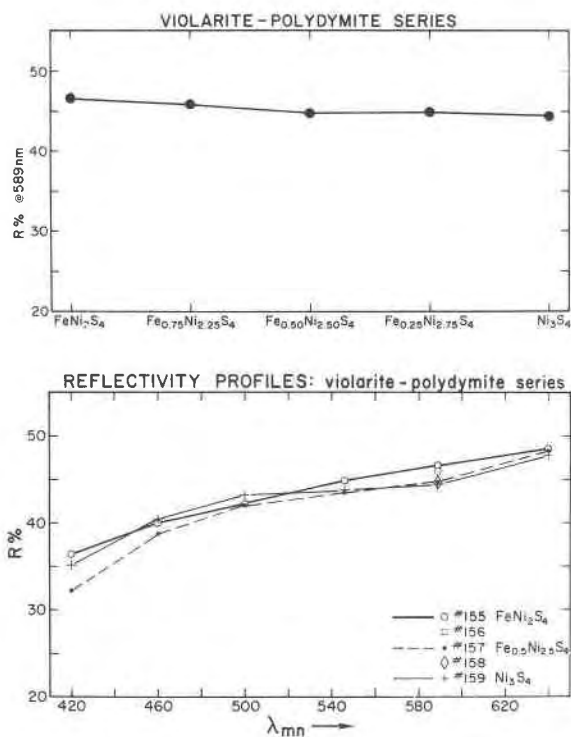
Fig. 3. Spectral reflectance data for violarites: (a) variation of reflectance at 589 nm with composition; (b) spectral reflectance curves for different compositions.
