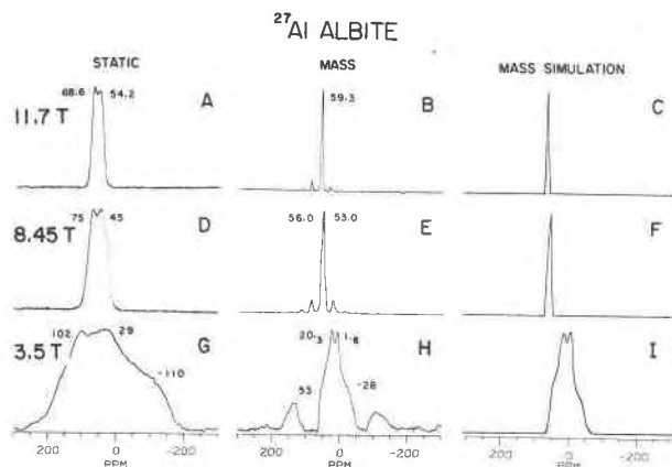
Fig. 6. ^{27}\text{Al} static and MASS NMR spectra of albite along with the MASS NMR computer simulations at 11.7, 8.45 and 3.5 Tesla. (A) 11.7 Tesla, static, 30 scans at 25 sec recycle time, 78 kHz spectral width, 3 \mu\text{sec} 90° pulse excitation, 4096 data points, 50 Hz linebroadening due to exponential multiplication. (B) 11.7 Tesla, 4.0 kHz MASS, 10 scans at 25 sec recycle time, 78 kHz spectral width, 3 \mu\text{sec} 90° pulse excitation, 8196 data points, 10 Hz linebroadening due to exponential multiplication. (C) 11.7 Tesla, MASS simulation, 65 Hz linebroadening. (D) 8.45 Tesla, static, 50 scans at 25 sec recycle time, 56 kHz spectral width, 3 \mu\text{sec} 90° pulse excitation, 4096 data points, 50 Hz linebroadening due to exponential multiplication. (E) 8.45 Tesla, 4 kHz MASS, 50 scans at 25 sec recycle time, 56 kHz spectral width, 3 \mu\text{sec} 90° pulse excitation, 8196 data points, 10 Hz linebroadening due to exponential multiplication. (F) 8.45 Tesla, MASS simulation, 150 Hz linebroadening. (G) 3.5 Tesla, static, 300 scans at 5 sec recycle time, 24 kHz spectral width, 3 \mu\text{sec} 90° pulse excitation, 4096 data points, 100 Hz linebroadening due to exponential multiplication. (H) 3.5 Tesla, 4 kHz MASS, 300 scans at 5 sec recycle time, 24 kHz spectral width, 3 \mu\text{sec} 90° pulse excitation, 4096 data points, 100 Hz linebroadening due to exponential multiplication. (I) 3.5 Tesla, MASS simulation, 100 Hz linebroadening.
