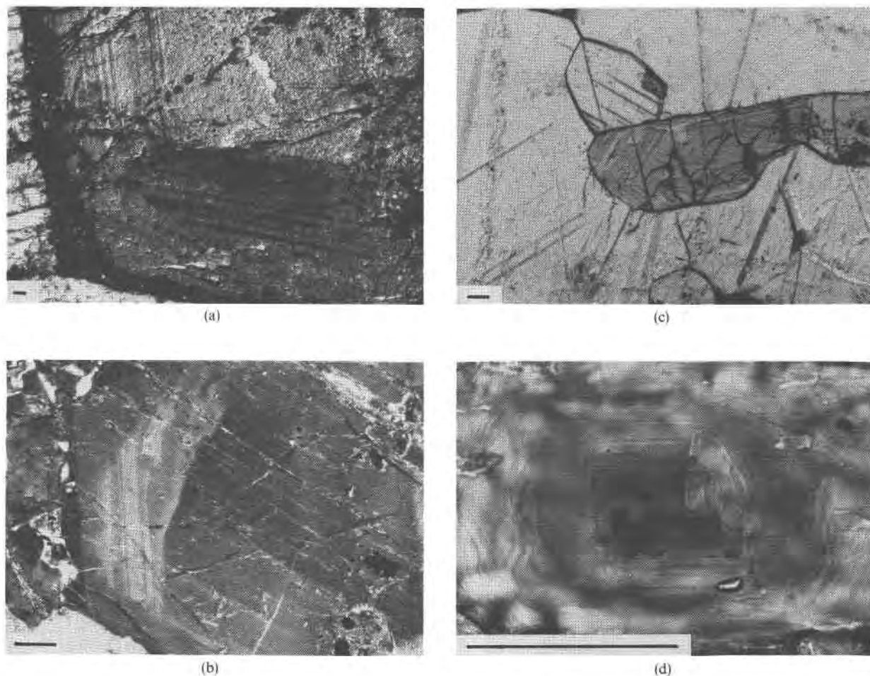
Fig. 5. Fine-scale optical zoning in pyroxenes from the JOMIC intrusion. Zonation corresponds to range of chemistry shown in Figures 7 and 8. Scale bars 0.1 mm. (a) Coarse-grained jacupirangite (790K9). Oblique illumination, plane light. (b) Fine-grained jacupirangite (790K12). Crossed polars. (c) Melilite-diopside carbonatite (790K23). Plane light. Other minerals are calcite (twin lamellae) and apatite. (d) Dopside melilitite (80B1-2). Plane light.
