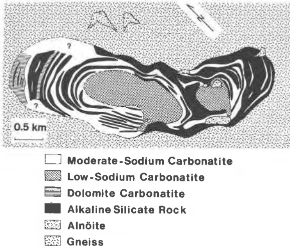
Fig. 1. Simplified geologic map of the Oka pluton, modified from Gold (1963, 1972) and Gold and Vallee (1969). The complex is emplaced into Grenville-age metamorphic rocks and is cut by alnöite breccia pipes. The complex is composed of four plutons in two intrusive centers, northern and southern. On the map, the two centers are not differentiated. At each intrusive center, the earlier pluton is a ring-complex of "moderate-alkali carbonatite" (containing the alkali-bearing silicate minerals melilite, nepheline, acmitic pyroxene, and/or alkali amphibole) and alkaline silicate rocks (jacupirangites, okaites, melilitites, ijolites and their alteration products). Cutting each ring-complex is a pluton of "low-alkali carbonatite" (containing no alkali-rich silicate minerals except phlogopite and/or hornblende). Sample locations shown are: A, Husereau Hill; B, Bond Zone; and C, Open Pit A2. See Appendix for exact sample locations.
