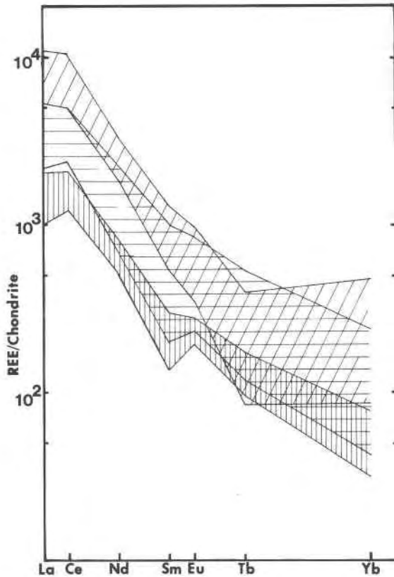
Fig. 4. Rare-earth element contents of Oka rocks, normalized to CI chondrites. Analyses by instrumental neutron activation. Key: melilite-diopside carbonatite, slanted hatchures; ijolite, vertical hatchure; and monticellite-diopside carbonatite, horizontal hatchure. High Yb values are probably in error.
