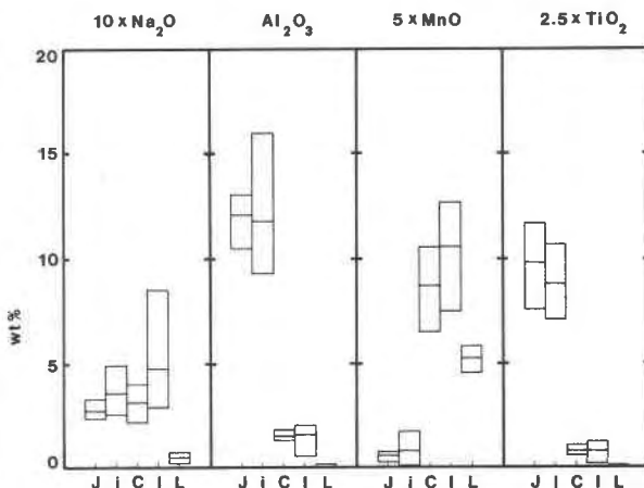
Fig. 7. Compositions of pyroxenes from the JOMIC pluton, plotted as ranges of minor-element contents (weight percent). Average is shown as central line within each bar. Key: J, coarse-grained jacupirangite; j, fine-grained jacupirangite; I, ijolite and diopside-melilitite; C, melilite-diopside carbonatite; L, monticellite-diopside carbonatite.
