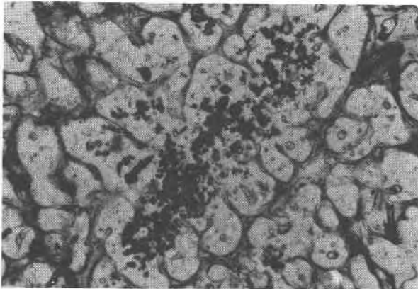
Fig. 1. Photomicrograph of Al-spinel (pleonaste-ferrian pleonaste) inclusions in leucite, glassy leucite lamproite, sample 71160408, Oscar Plug. Note irregular shape of aggregated leucite phenocrysts. Width of field is 0.55 mm.
