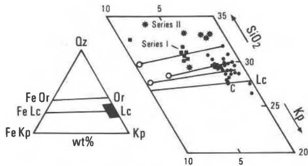
Fig. 4. Compositions of leucites in the West Kimberley lamproites (dots) compared with experimental leucite compositions in the system \text{SiO}_2\text{-KFe}^{3+}\text{SiO}_4\text{-KAlSiO}_4 (after Carmichael, 1967). Squares = first series experiments; crosses = second series experiments; open circles = bulk scans of Al-spinel plus leucite host in West Kimberley lamproites.
