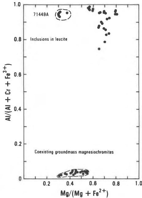
Fig. 3. Compositions of aluminous spinel inclusions in leucite in West Kimberley leucite lamproites contrasted with groundmass titanian magnesiochromites in terms of Al/(Al + Cr + Fe 3+ ) versus Mg/(Mg + Fe 2+ ).
