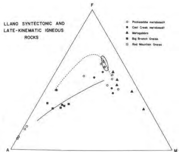
Fig. 5. Alkali- FeO^*-MgO (AFM) diagram for the syntectonic and late-kinematic metaigneous rock suite of the Llano Uplift, Texas. Solid line outlines the trend for the Cascades province, northwestern U.S. (Carmichael et al., 1974). Dashed line outlines the trend for the island arc suite from Tonga (Ringwood, 1975). Stippled area is Packsaddle Schist amphibolites (Garrison, 1981b). Weight percent oxides used for plot.
