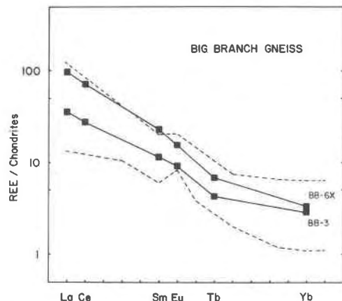
Fig. 8. Plot of chondrite-normalized REE abundances for two samples of Big Branch Gneiss. Dashed lines outline the range of tonalites and trondhjemites from Finland and Norway (Arth and Barker, 1976).
