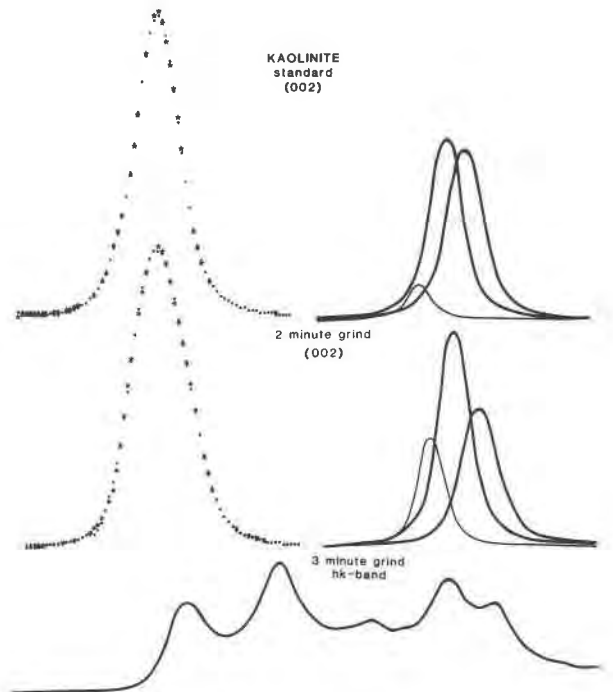
Fig. 7. Duplicate patterns for standard and 2-minute grind (002) profiles and 3 minute grind hk -band.
