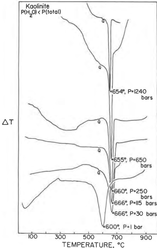
Fig. 2. Representative DTA patterns of kaolinite (KGa-I) for open capsule runs without added water. Note that the peaks become sharper with increasing pressure. (Q = Quartz).
