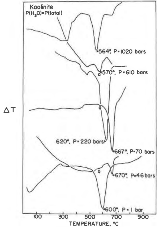
Fig. 3. Representative DTA patterns of kaolinite (KGa-I) for closed capsule runs with added water. Although the peaks become sharper with increasing pressure, peak widths are significantly different than those shown in Fig. 2. All runs made with the recorder at the 50 μv range, except the 610 bar run, which was made at the 100 μv range.
