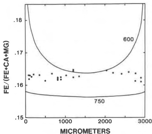
Fig. 6. Compositional data from electron microprobe analyses along a diameter of a garnet crystal in Jagersfontein nodule J34, compared with calculated compositional profiles for a garnet of similar size. The profiles are calculated for 750 and 600°C temperatures of a linear cooling history beginning at 1100°C, using the diffusion parameters of Set A. The absolute levels of the calculated profiles are not meaningfully related to the actual garnet composition. Rather, the calculated profiles show the extent and degree of curvature expected as cation profiles are frozen in during cooling. The scatter of the duplicated compositional measurements is due to counting statistics and instrumental drift, and the scatter can be used to assess the precision with which homogeneity is defined.
