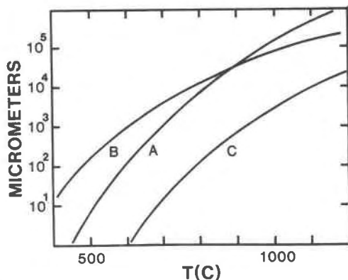
Fig. 5. Curves show effective diffusion distances in \mu\text{m} for linear cooling of 1°C per million years through 100°C intervals. Each curve is drawn through points plotted at the midpoints of 100°C intervals: the points were calculated from the square roots of the products of diffusivity and time, calculated by numerical integration over the 100°C intervals, using the diffusion parameters of Sets A, B, and C in Table 1.
