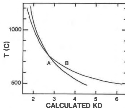
Fig. 1. Dependence of K_D (Fe/Mg in garnet divided by Fe/Mg in olivine) upon temperature, as calculated from the algorithms of O'Neill and Wood (1979) (Curve A) and of Kawasaki (1979) (Curve B). K_D values were calculated for olivine with 6 mole percent fayalite, garnet with Ca/(Ca+Fe+Mg) of 0.137 and a pressure of 25 kbar.
