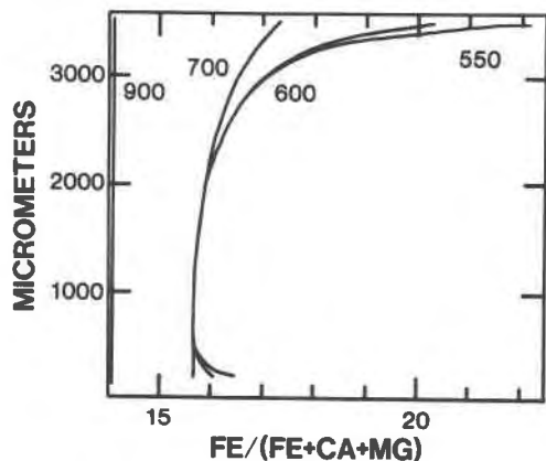
Fig. 3. Calculated compositional profiles in garnet for a cooling history beginning at 1200°C in a slab with a surface temperature of 500°C and with the diffusion parameters of Set A. The garnet extends from a central olivine inclusion (radius 230 \mu\text{m} ) to the outer olivine shell which begins at 3500 \mu\text{m} . Profiles are shown at 900, 700, 600, and 550°C.
