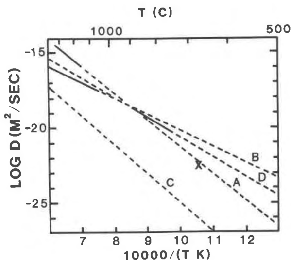
Fig. 2. Lines show the calculated diffusion coefficients as functions of temperature, according to the four sources discussed in Table 1. The solid portions of the lines show the temperature ranges of the experimental studies. The "X" shows an estimate of Lasaga et al. (1977) for a crustal garnet.
