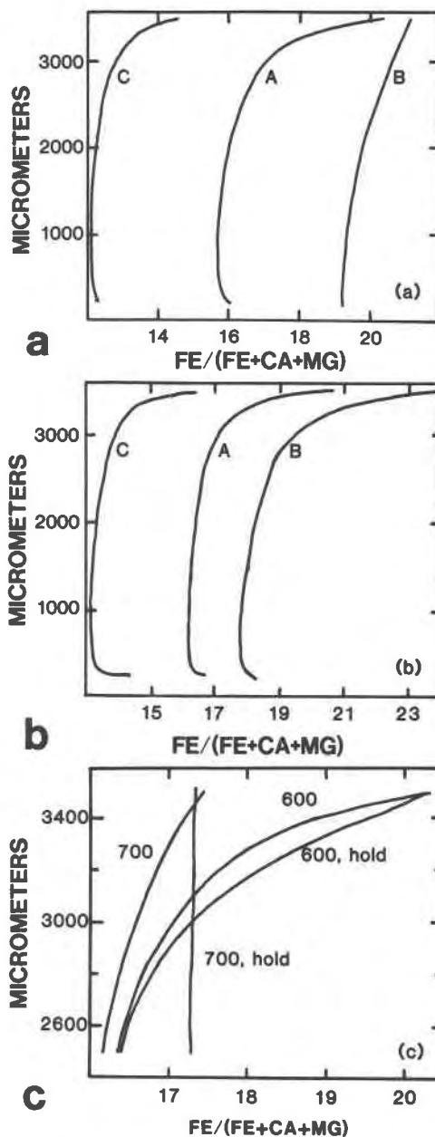
Fig. 4. Comparisons of numerical experiments with different garnet diffusion parameters and cooling histories. (A) Compositional profiles in garnet for the cooling slab model, using the diffusion parameters of Set A (at 600°C), Set B (at 550°C), and Set C (at 900°C) (B) Compositional profiles in garnet for linear cooling at 1°C per million years, using the diffusion parameters of Set A (600°C), Set B (600°C) and Set C (500°C). (C) Comparisons of compositional profiles before and after annealing at constant temperature for 500 million years. Though the model garnet was 3500 \mu\text{m} in radius, profiles are shown only for the outer 1000 \mu\text{m} . One pair of lines shows results for first cooling to 700°C and then for holding 500 million years at that temperature; homogenization is complete after the annealing time. In contrast, the profile produced after cooling to 600°C is nearly unaffected by the subsequent annealing. Profiles were calculated using the diffusion parameters of Set A.
