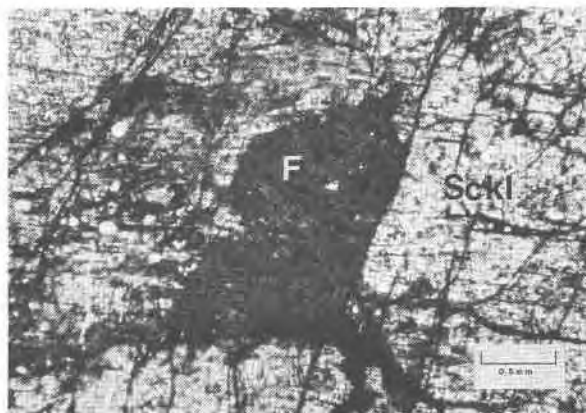
Fig. 9. Photomicrograph of reddish-brown phase 'F' (F) in massive, yellow sicklerite (sck1). Plain light.
