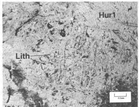
Fig. 5. Photomicrograph showing the alteration of lithiophilite (lith) to hureaulite I (hur1). The lithiophilite appears as colorless, high-relief grains surrounded by colorless hureaulite and other minor secondary phosphates. Plain light.
