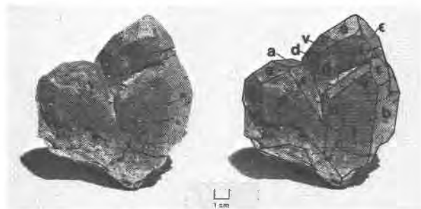
Fig. 4. Photograph and superimposed drawing of a lithiophilite crystal group from the Stewart Lithia mine. The group consists of several intergrown crystals oriented in a parallel fashion. Crystal faces are outlined and are identified by conventional letter designations (see text).
