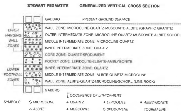
Fig. 2. Generalized vertical cross section through the southern portion of the Stewart pegmatite illustrating the mineral assemblages that comprise the internal zoning structure.
