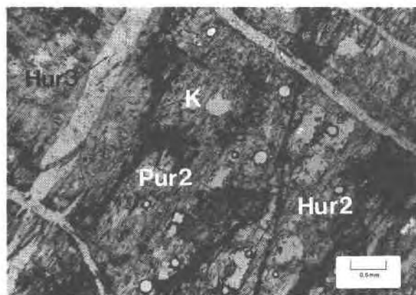
Fig. 7. Photomicrograph of massive, pale green hureaulite II (hur2) containing small areas of violet-red purpurite II (pur2), greenish-yellow veinlets of phase ‘K’ (K), and transected by later veinlets of colorless hureaulite III (hur3). Plain light.
