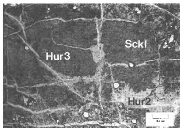
Fig. 6. Photomicrograph of massive, yellow sicklerite (sck1) being replaced by pale green hureaulite II (hur2). Both minerals are cut by narrow veinlets of colorless hureaulite III (hur3). Plain light.
