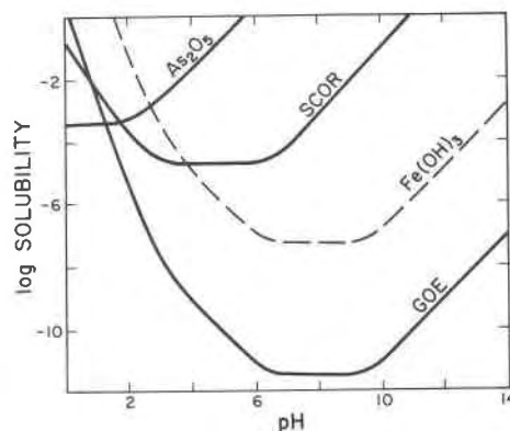
Fig. 6. Logarithm of solubility versus pH for \text{As}_2\text{O}_5 , scorodite, amorphous \text{Fe}(\text{OH})_3 and goethite. The goethite and \text{Fe}(\text{OH})_3 curves were derived from data given in Stumm and Morgan (1981, p. 780). The \text{As}_2\text{O}_5 curve was derived from data given by Naumov (1974). The scorodite curve was derived from the K_{\text{sp}} determined in this study.
