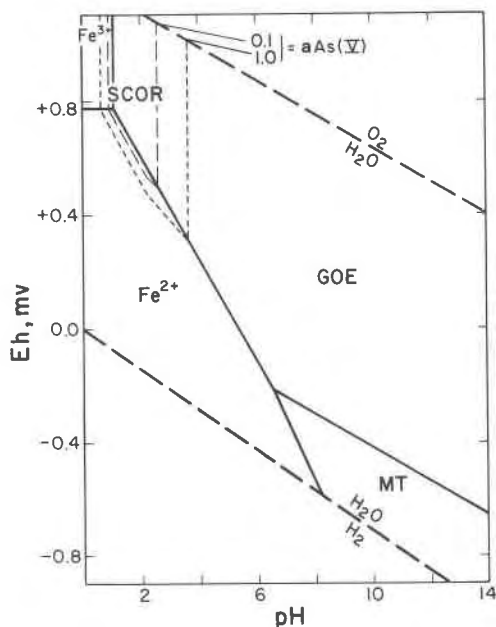
Fig. 5. Eh-pH relations for the Fe-H 2 O system at a_{\text{Fe}} = 10^{-3} (solid lines). The arsenate-H 2 O system is superimposed on this diagram. Scorodite is stable when arsenate activities are greater than or equal to 10^{-1.29} .
