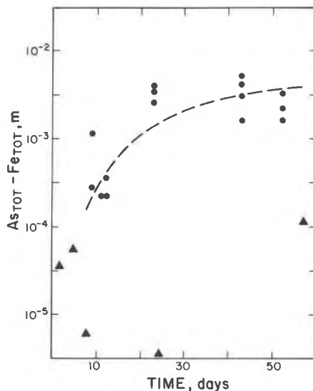
Fig. 2. Total arsenic concentration minus total iron concentration versus time for all experiments. Triangles denote experiments in which scorodite dissolved congruently. Dots represent experiments in which incongruent dissolution was predominant.
