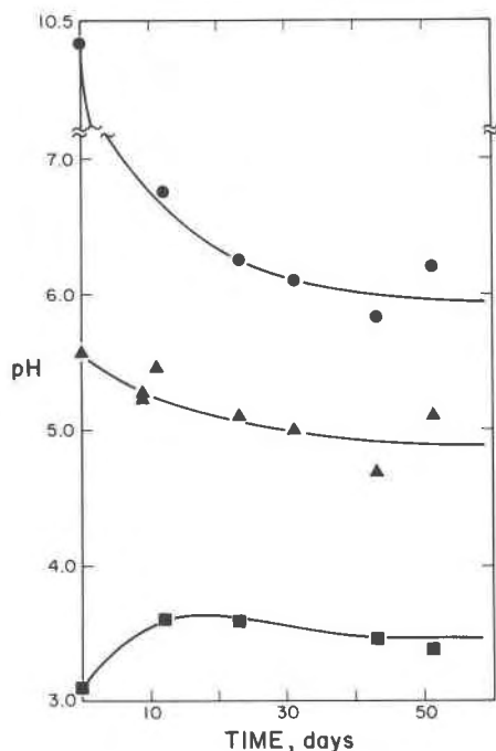
Fig. 3. pH versus time, showing the systematic pH change for experiments with three different initial pH conditions. Dots represent the high pH group, initial pH = 10.38; triangles represent the intermediate pH group, initial pH = 5.57; squares represent the low pH group, initial pH = 3.08. The reactions causing the systematic variations of pH with time are explained in the text. Data used in this diagram are from Dove (1984).
