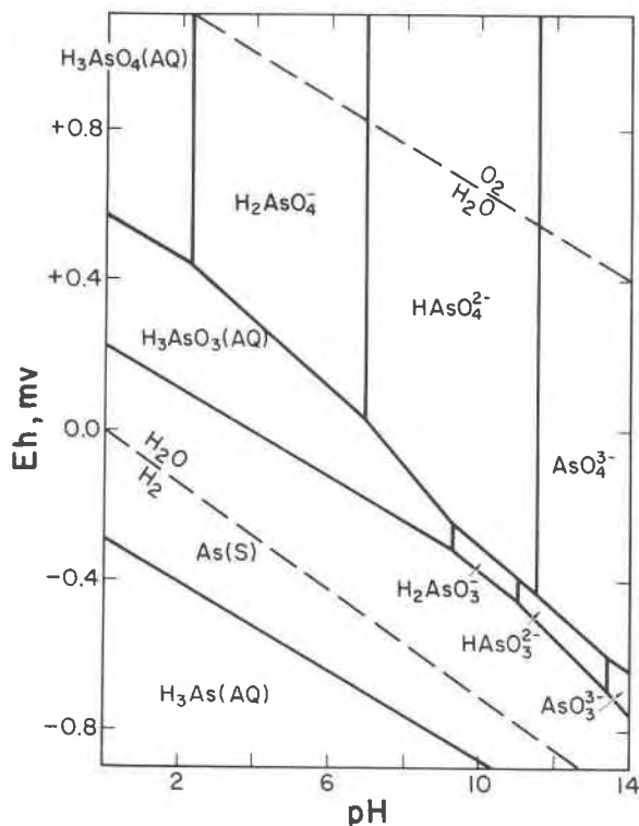
Fig. 1. Eh-pH diagram of the arsenic-H 2 O system at a_{\text{As}} = 10^{-3} . Derived from the program SOLUPLLOT (Bethke, 1978).
