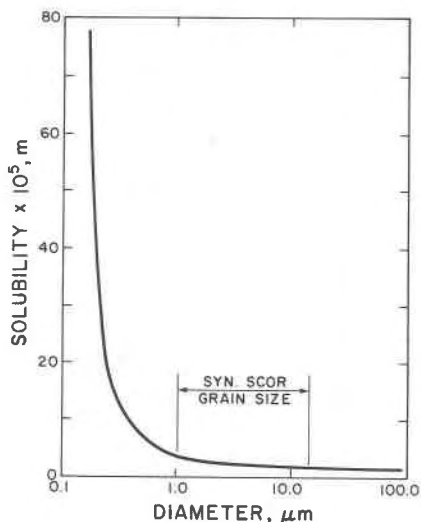
Fig. 4. Scorodite solubility as a function of grain diameter, as calculated from equation (10).
