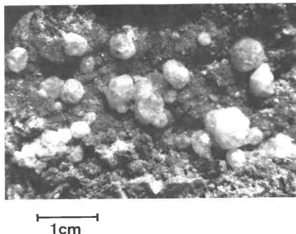
Fig. 1. Ammonioleucite, shown as white surface layers replacing trapezohedral analcime crystals.
