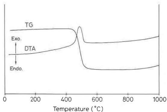
Fig. 4. DTA and TG curves of ammonioleucite.
