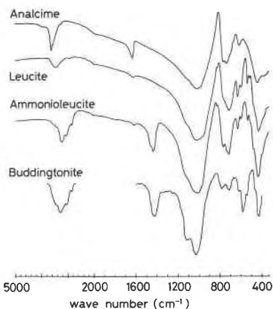
Fig. 3. Infrared absorption spectra of ammonioleucite. Those of analcime, leucite, and buddingtonite are also given for comparison (that for buddingtonite from Loughnan et al. , 1983).
