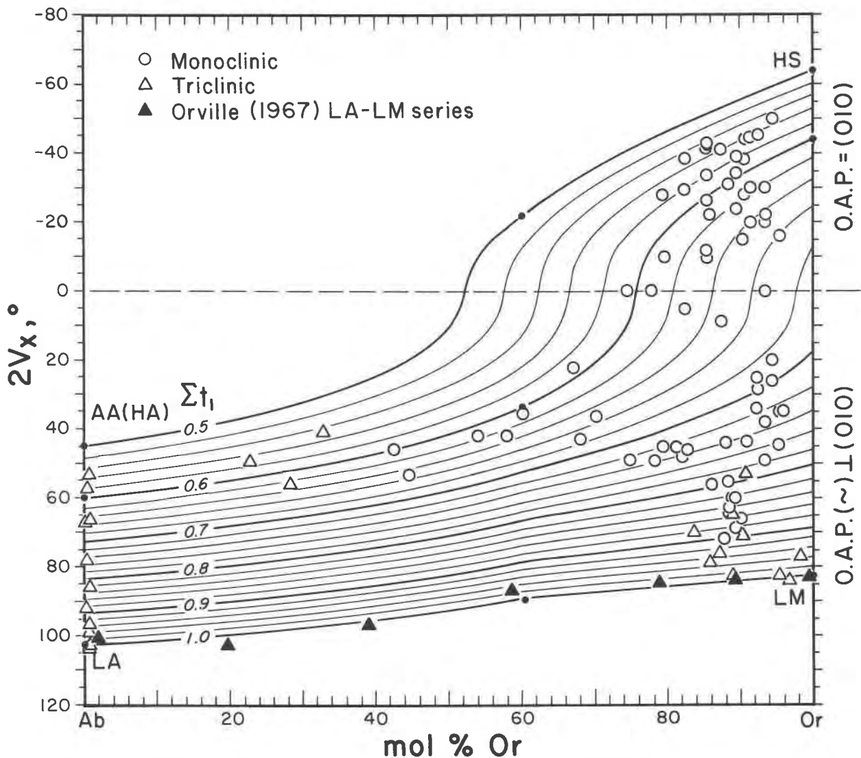
Fig. 2. Plot of 2V_x versus mole percent Or contoured for \Sigma t_1 : AA = analbite, i.e., a disordered albite with t_{1o} = t_{1m} and t_{2o} = t_{2m} , which will invert to monoclinic symmetry at temperatures above 980^\circ\text{C} ; other symbols as elsewhere in text. The 109 data from Table 1 are plotted here. Solid triangles represent the largest 2V_x value measured by Rankin (1967) on each of the compositions in the LA-LM alkali-exchange series of Orville (1967).
