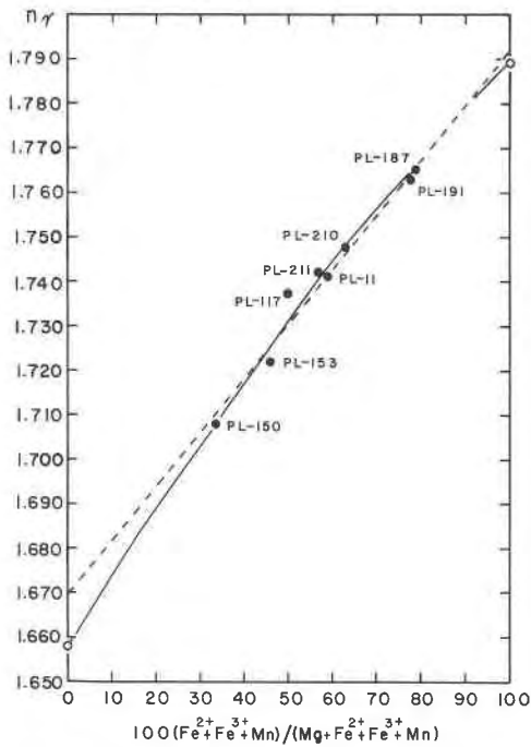
Fig. 2. The ratio 100(\text{Fe}^{2+} + \text{Fe}^{3+} + \text{Mn})/(\text{Mg} + \text{Fe}^{2+} + \text{Fe}^{3+} + \text{Mn}) versus n_x for Ca-poor pyroxenes from Puttuualuk Lake area. Dashed line is result of linear regression analysis with r^2 = 0.969 . The equation for this line is n_x = 0.1235[(\text{Fe}_i + \text{Mn})/(\text{Mg} + \text{Fe}_i + \text{Mn})] + 1.6689 . Solid curve is visually fit to the data. Open circles are indices of synthetic enstatite (1.658) and orthoferrosilite (1.789) from Stephenson et al. (1966) and Lindsley et al. (1964), respectively.
