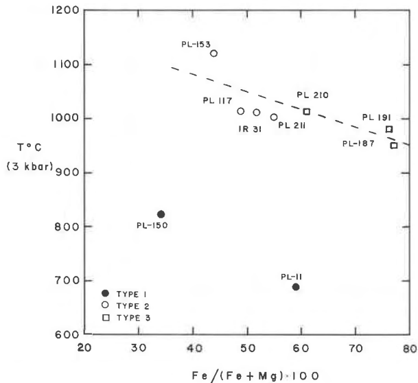
Fig. 8. Temperature of crystallization at 3-kbar pressure plotted against 100\text{Fe}/(\text{Fe} + \text{Mg}) for Puttuaaluk Lake pyroxenes. Pyroxene bulk compositions were reconstructed from host and lamellar compositions as described in the text, with the exception of PL-11 and PL-150, which contain only fine (100) augite exsolution. Temperatures are minimum temperatures except for PL-11 and PL-187, which are saturated with augite. High-temperature crystallization trend is that of Type 2 and Type 3 pyroxenes. Dashed line is visually fit to the data. Pyroxenes from PL-11 and PL-150 plotting at low temperature are Type 1 pyroxenes. See text for discussion.
