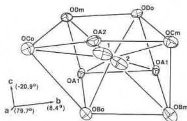
Fig. 2. Perspective view of the M-site environment from the final X-ray structure of no. 299B plagioclase (ORTEP plot, 98% probability ellipsoids). Orientation of the unit-cell axes is indicated at the lower left. Angle of inclination to the projection plane is shown for each axis with a positive angle denoting that the positive end of the corresponding axis lies above the projection plane. The unit-cell origin lies on the OA1-OA1 join. Labels 1 and 2 denote, respectively, atoms M' and M''.
