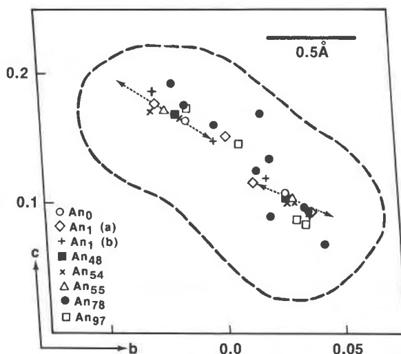
Fig. 3. M-site positions of various plagioclases converted to C\bar{1} cell coordinates and projected parallel to the a axis onto a b-c section. Data have been taken from \text{An}_0 —Winter et al. (1979), 2-site model; \text{An}_1 (a)—Ribbe et al. (1969), 4-site model; \text{An}_1 (b)—Prewitt et al. (1976); \text{An}_{48} —this study; \text{An}_{54} —Korekawa et al. (1979); \text{An}_{55} —Toman and Frueh (1976b); \text{An}_{78} —Kitamura and Morimoto (1977); and \text{An}_{97} —Czank et al. quoted by Smith (1974, vol. 1, p. 138). The two dashed arrows represent the projection of the displacement modulation wave vectors refined for both M positions of an \text{An}_{55} structure by Toman and Frueh (1976b). The heavy dashed line encircling the plot is the first positive contour from the difference Fourier section of Fig. 1a.
