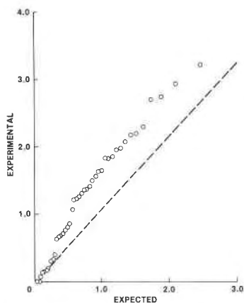
Fig. A1. Half-normal probability plot for refined positional parameters of plagioclase no. 299B. The dashed line represents an ideal normal distribution of \delta p_i . The linearity of the experimental points indicates that the \delta p_i is approximately normally distributed.
