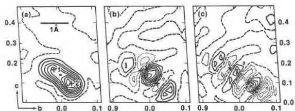
Fig. 1. Difference Fourier sections through the no. 299B plagioclase M site. All plots are b - c sections at a = 0.26 for various stages of X refinement. See text for details; section (a) was computed during refinement stage 3, (b) during stage 4, and (c) following stage 5. Contour intervals (in electrons/Å 3 ) for these sections are (a) 2.349, (b) 0.830, and (c) 0.154. Lines representing negative contours are dotted, those for zero contours are dashed, and those for positive contours are solid. Label 1 identifies the final refined position of atom M', 2 likewise for M''.
