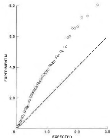
Fig. A2. Half-normal probability plot for plagioclase no. 299B refined thermal parameters. (Note that the slope of the reference line here equals 2). The deviation from linearity of experimental points suggests that some systematic bias exists between the X-ray and neutron thermal parameters.
