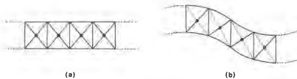
Fig. 5. The effect of layer modulation, producing an axial elongation of the Cu octahedra of the \alpha -PbO 2 type chains. Of course, the modulation actually occurs because of the spontaneous distortion of the octahedra rather than vice versa.
