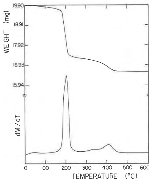
Fig. 2. Thermogravimetric analysis of the S(24) sample. dM/dT = mass variation/temperature variation.
