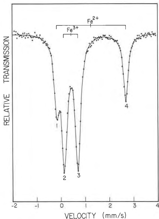
Fig. 1. Mössbauer spectrum of the S(10) powder sample at room temperature (velocity relative to metallic iron).
