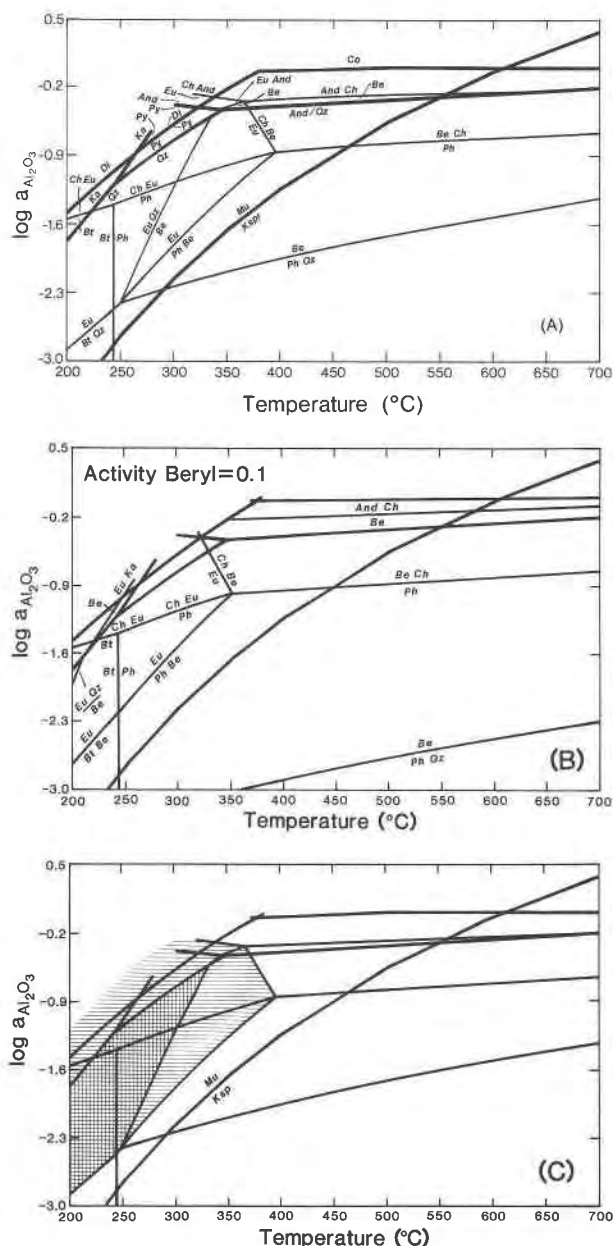
Fig. 12. Log a_{\text{Al}_2\text{O}_3} -temperature projection of BASH phase relations at 1 kbar. (A) Calculated phase relations for the pure system. Also shown is the curve for the reaction muscovite = K-feldspar + alumina + water. (B) Calculated phase relations for a_{\text{beryl}} = 0.1 . The curves are the same as in (A) except where labeled. Note the effect of the expansion of the beryl stability fields. (C) Projection of the stability fields of euclase (horizontally ruled) and euclase + quartz (vertically ruled) with a_{\text{beryl}} = 1 . The curves are the same as in (A). Note that euclase is incompatible with K-feldspar. See text for further discussion. Abbreviations from Table 1.
