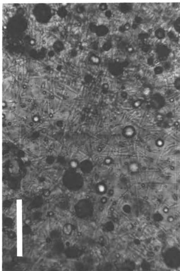
Fig. 2. Photomicrograph of dendritic groups of interlocking quartz crystals together with vapor bubbles in aluminosilicate glass from run capsule 1–9. Scale bar = 100 \mu\text{m} .
