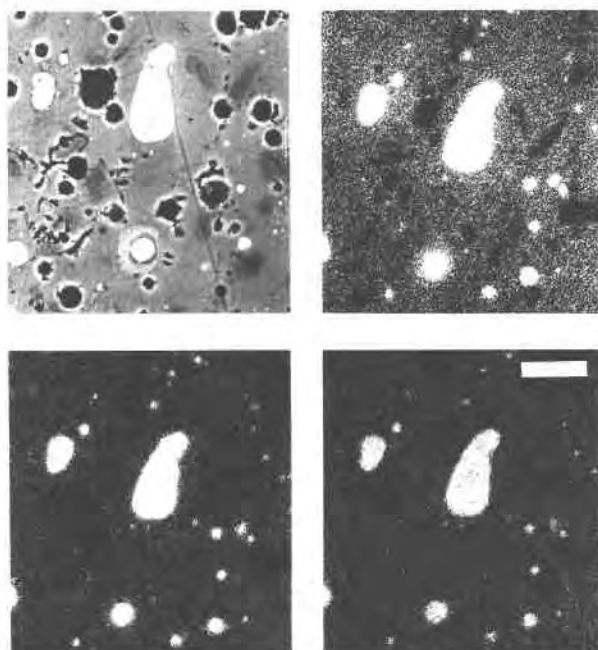
Fig. 4. Back-scattered electron photomicrograph (upper left) and corresponding K\alpha X-ray maps for phosphorus (upper right), manganese (lower left), and iron (lower right) for lithiophilite grains in aluminosilicate glass from run capsule 2-3 (see Fig. 3). Scale bar, applicable to all four images, equals 25 \mu\text{m} . The white, irregular blebs are lithiophilite-triphylite crystals. The dark-gray objects within the glass shown in the back-scattered electron micrograph are quartz crystals, and the black features are holes formed by vapor bubbles. The sharp lines in this photomicrograph are scratches on the glass surface caused by polishing.
