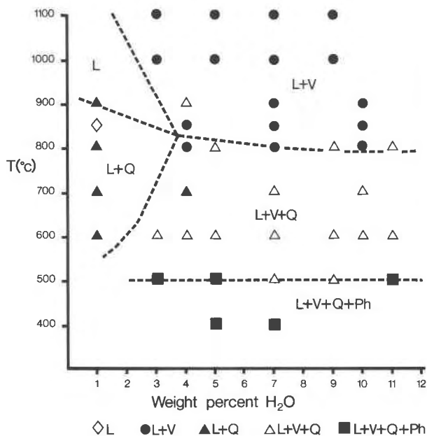
Fig. 1. Pseudobinary temperature-composition diagram showing the phase assemblages in the run products from 12 crystallization experiments. Boundaries separating phase-assemblage fields are marked by dashed lines and are believed to be accurate to \pm 50^\circ\text{C} and \pm 0.5 wt% \text{H}_2\text{O} . The letters refer to the following phases: L = liquid (melt), V = vapor, Q = quartz, Ph = phosphate (primarily lithiophilite-triphyllite).
