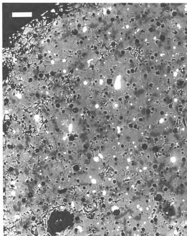
Fig. 3. Back-scattered electron photomicrograph of a polished thin section of aluminosilicate glass from run capsule 2-3. Grains of the Mn-Fe phosphate mineral identified as lithiophilite appear as white, spherical-, irregular-, or equant-shaped areas distributed throughout the glass. The dark-gray areas within the glass represent tabular quartz crystals. Scale bar = 50 \mu\text{m} .
