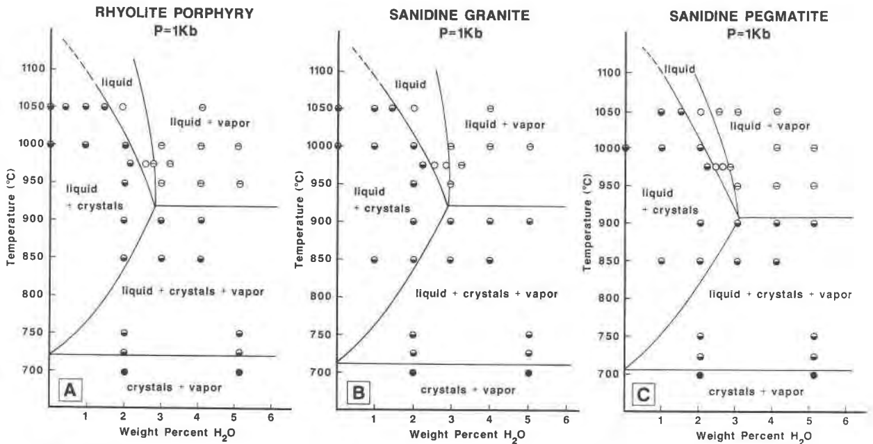
Fig. 10. Experimentally determined stability fields for (A) rhyolite porphyry, (B) sanidine granite, and (C) sanidine pegmatite are very similar at 1-kbar total confining pressure. In these “pseudo-binary” projections of temperature vs. percent H 2 O added to the anhydrous natural starting materials, the vapor-saturated liquidus is between 900 and 950° and the solidus between 700 and 725°. Stability fields for phase assemblages are individually labeled.
