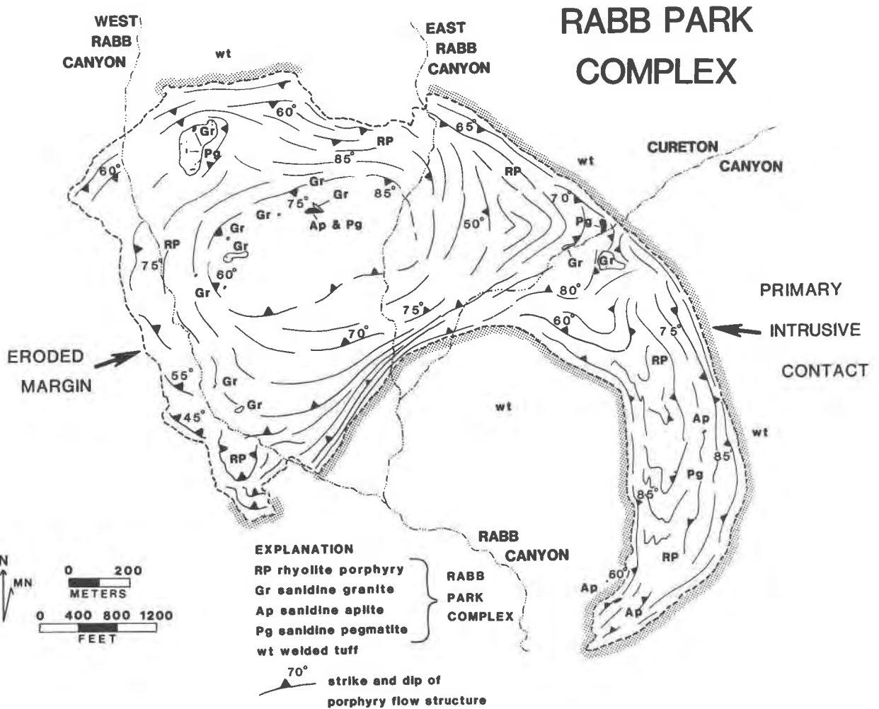
Fig. 3. Flow structures within the main rhyolite porphyry mass wrap around scattered inclusions of granite, aplite, and pegmatite.
