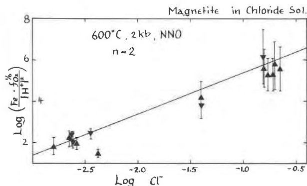
Fig. 16. Solubility of magnetite in HCl-NaCl-H 2 O solutions as a function of free chloride ion molality at 600°C, 2 kbar, and f_{O_2} controlled by NNO. The solid line is drawn with a slope of 2, indicating that FeCl 2 is the dominant solute. From Wang and Eugster (in prep.).
