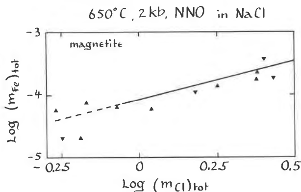
Fig. 17. Solubility of magnetite in NaCl-H 2 O solutions at 650°C, 2 kbar, and f_{O_2} controlled by NNO, drawn as a function of total chloride molality. From Wang and Eugster (in prep.).
