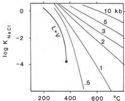
Fig. 6. Dissociation constant of NaCl in water vapor as a function of temperature (°C). Isobars have been contoured in kilobars. From the data of Quist and Marshall (1968).
