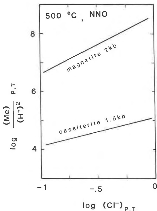
Fig. 23. Comparison of the solubility of magnetite and cassiterite in HCl-H 2 O solutions, 500°C, 2 kbar (magnetite), 1.5 kbar (cassiterite) and f_{O_2} controlled by NNO. The slopes of the lines are 2 and 1, corresponding to FeCl 2 and SnCl + , respectively. Data from Chou and Eugster (1977) and Wilson (1986).
