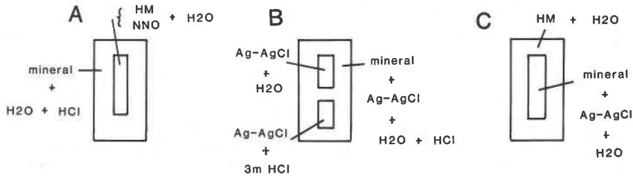
Fig. 15. Experimental arrangements for supercritical speciation determinations from mineral solubilities. (A) Method of Wilson (1986). See also Wilson and Eugster (1984, 1985), Eugster and Wilson (1985), Eugster et al. (1986). (B) "Unbuffered" or "modified buffer" method of Frantz and Popp (1979) and Doctor et al. (1980). (C) Ag-AgCl buffer method of Frantz and Eugster (1973). For details see text.
