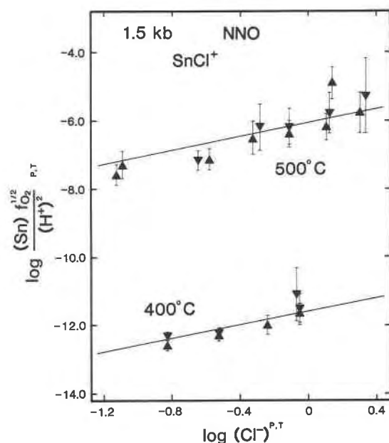
Fig. 18. Solubility of cassiterite in HCl-H 2 O solutions, as a function of chloride ion molality at 400 and 500°C, 1.5 kbar, and f_{O_2} controlled by NNO. The solid lines have a slope of 1, indicating that SnCl + is the dominant solute. From Wilson (1986).
