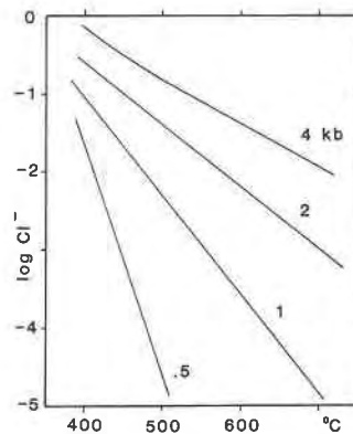
Fig. 9. Molality of free chloride ions for a 0.1-molar solution of HCl-H 2 O as a function of temperature (°C). Pressure is contoured in kilobars.
