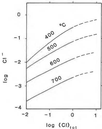
Fig. 7. Molality of free chloride ions as a function of total chloride concentration in NaCl-H 2 O solutions at 1-kbar pressure. Isotherms are contoured in °C.
