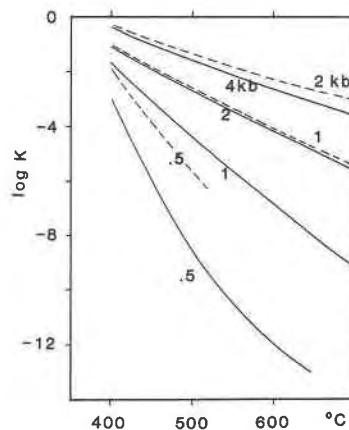
Fig. 8. Dissociation constant of HCl as a function of temperature (°C). Pressure is contoured in kilobars. From the data of Frantz and Marshall (1984). For comparison, the NaCl data of Figure 6 are shown as dashed curves.
