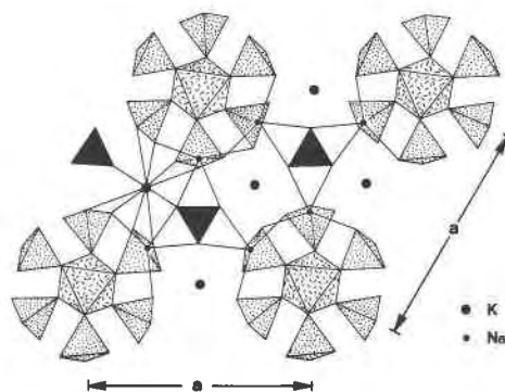
Fig. 2. The structure of ungemachite viewed down [001]. (FeO 6 ) octahedra are dashed, (SO 4 ) tetrahedra are dotted, (NO 3 ) triangles are black. Note the prominent [(Fe 3+ (SO 4 ) 6 )] finite clusters that constitute the fundamental building block of the structure.
