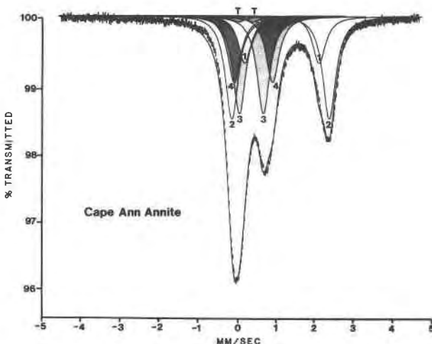
Fig. 8. Mössbauer spectrum of annite from the type locality at Cape Ann, Massachusetts (specimen 14); peaks 1-1— \text{Fe}^{2+}_{\text{oct}} in trans -M1; peaks 2-2— \text{Fe}^{2+}_{\text{oct}} in cis -M2; peaks 3-3— \text{Fe}^{2+}_{\text{oct}} in cis -M2; peaks 4-4— \text{Fe}^{2+}_{\text{oct}} in trans -M1; peaks T-T— \text{Fe}^{3+}_{\text{tet}} .
