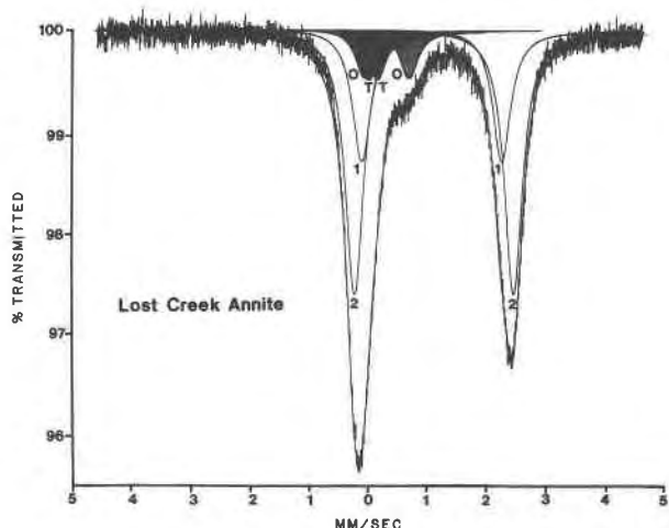
Fig. 7. Mössbauer spectrum of annite from Lost Creek, Montana (specimen 12); peaks 1-1— \text{Fe}^{2+}_{\text{oct}} in trans -M1; peaks 2-2— \text{Fe}^{2+}_{\text{oct}} in cis -M2; peaks T-T— \text{Fe}^{3+}_{\text{tet}} ; peaks 0-0— \text{Fe}^{3+}_{\text{oct}} .
