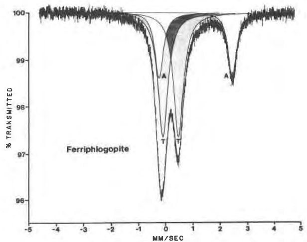
Fig. 5. Mössbauer spectrum of ferriphlogopite (specimen 8). The spectrum is dominated by peaks due to tetrahedral \text{Fe}^{3+} ions; peaks A-A— \text{Fe}_{\text{oct}}^{2+} ; peaks T-T— \text{Fe}_{\text{tet}}^{3+} .
