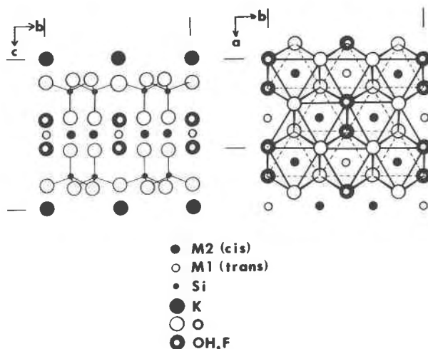
Fig. 1. Schematic diagram of the mica crystal structure. (left) Projected onto (100) showing the locations of the cation sites and OH - anions. (right) Projected onto (001), showing the configurations of the cis -M2 and trans -M1 coordination polyhedra.
