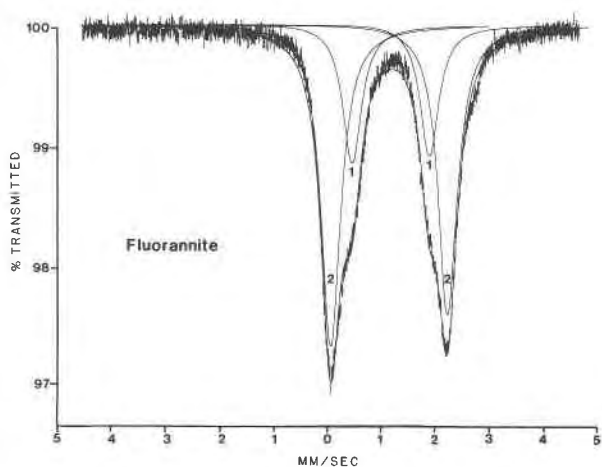
Fig. 9. Mössbauer spectrum of synthetic fluorannite (specimen 15); peaks 1-1— \text{Fe}^{2+}_{\text{oct}} in trans -M1; peaks 2-2— \text{Fe}^{2+}_{\text{oct}} in cis -M2.
