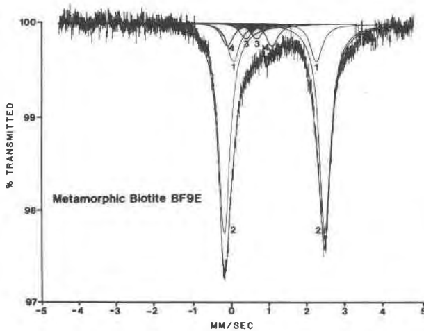
Fig. 4. Mössbauer spectrum of metamorphic biotite BF9E (specimen 6); peaks 1-1— \text{Fe}_{\text{oct}}^{2+} in trans -M1; peaks 2-2— \text{Fe}_{\text{oct}}^{2+} in cis -M2; peaks 3-3— \text{Fe}_{\text{oct}}^{3+} in cis -M2; peaks 4-4— \text{Fe}_{\text{oct}}^{3+} in trans -M1.
