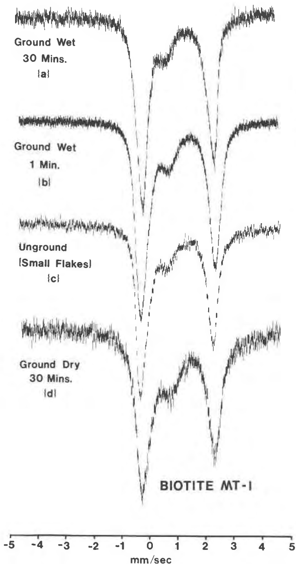
Fig. 2. Mössbauer spectra of biotite MT-1 (specimen 1) prepared in different ways. Spectra (a), (b), and (c) are remarkably similar, but spectrum (d) shows an enlarged \text{Fe}^{3+} peak around 1 mm/s resulting from oxidation during dry grinding of the biotite specimen.
