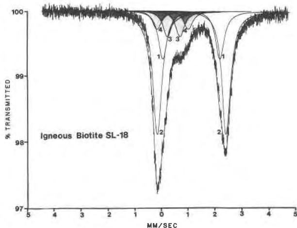
Fig. 3. Mössbauer spectrum of igneous biotite SL-18 (specimen 2); peaks 1-1— \text{Fe}^{2+} in trans -M1; peaks 2-2— \text{Fe}^{2+} in cis -M2; peaks 3-3— \text{Fe}^{3+} in cis -M2; peaks 4-4— \text{Fe}^{3+} in trans -M1.
