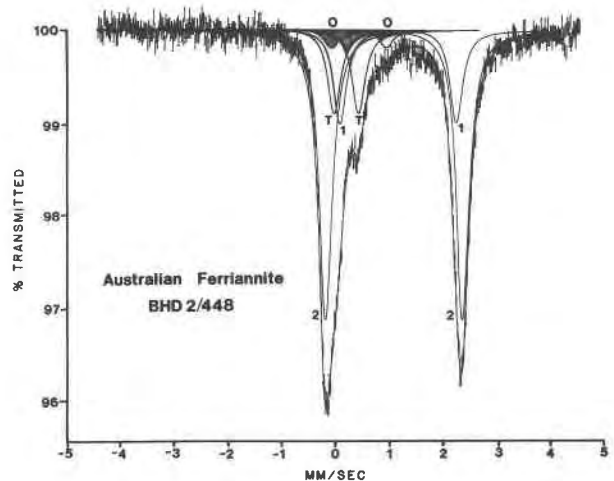
Fig. 6. Mössbauer spectrum of ferriannite BHD2/448 (specimen 10) from a banded iron formation. The majority of \text{Fe}^{3+} ions are in tetrahedral sites; peaks 1-1— \text{Fe}_{\text{oct}}^{2+} in trans -M1; peaks 2-2— \text{Fe}_{\text{oct}}^{2+} in cis -M2; peaks T-T— \text{Fe}_{\text{tet}}^{3+} ; peaks 0-0— \text{Fe}_{\text{oct}}^{3+} .
