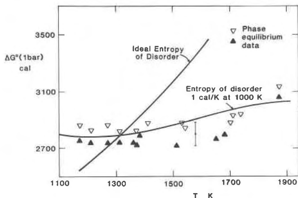
Fig. 4. Same experimental data as Fig. 4 recalculated to \Delta G_{\text{bar}}^{\circ} for Reaction 3. Arrows indicate direction of "true" \Delta G_{\text{bar}}^{\circ} at the temperature of interest. Error bar gives approximate uncertainty in \Delta G values derived from high-pressure experiments. About 1 cal/K of residual disorder is required by the experimental data.
