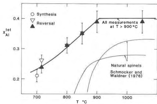
Fig. 2. Measured degree of inversion of MgAl_2O_4 spinel as a function of temperature. Note that all experiments at T > 900^\circ C give the same amount of tetrahedral Al (0.39 approx., Table 1). Open and closed triangles refer, respectively, to equilibrium approached from high X_{Al}^{tet} and low X_{Al}^{tet} . Data of Schmocker and Waldner are ESR measurements of Cr^{3+} -bearing natural spinels (see text).
