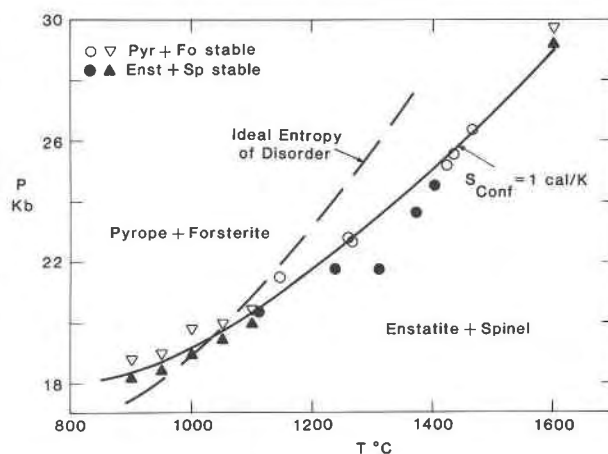
Fig. 3. Experimental data on the reaction enstatite + spinel = pyrope + forsterite. \circ \bullet Perkins et al. (1981). \nabla \blacktriangle Danckwerth and Newton (1978) (900–1100°C) and Gasparik and Newton (1984) (1600°C). Open symbols, Pyr + Fo stable; solid symbols, Enst + Sp stable. Curve labeled "ideal entropy of disorder" assumes a residual entropy of 2.6 cal/K. Solid curve is calculated for a residual entropy of 1 cal/K.
