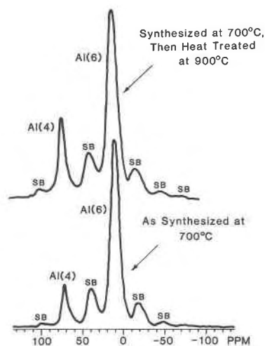
Fig. 1. High-resolution 11.7-T MASS NMR spectra of spinel synthesized at 700°C (lower) and of the same sample heat treated for 8 d at 900°C (upper). Note marked increase in intensity of major tetrahedral peak at 900°C. Al(4) denotes tetrahedral Al, Al(6) denotes octahedral Al, and SB denotes spinning sidebands.
