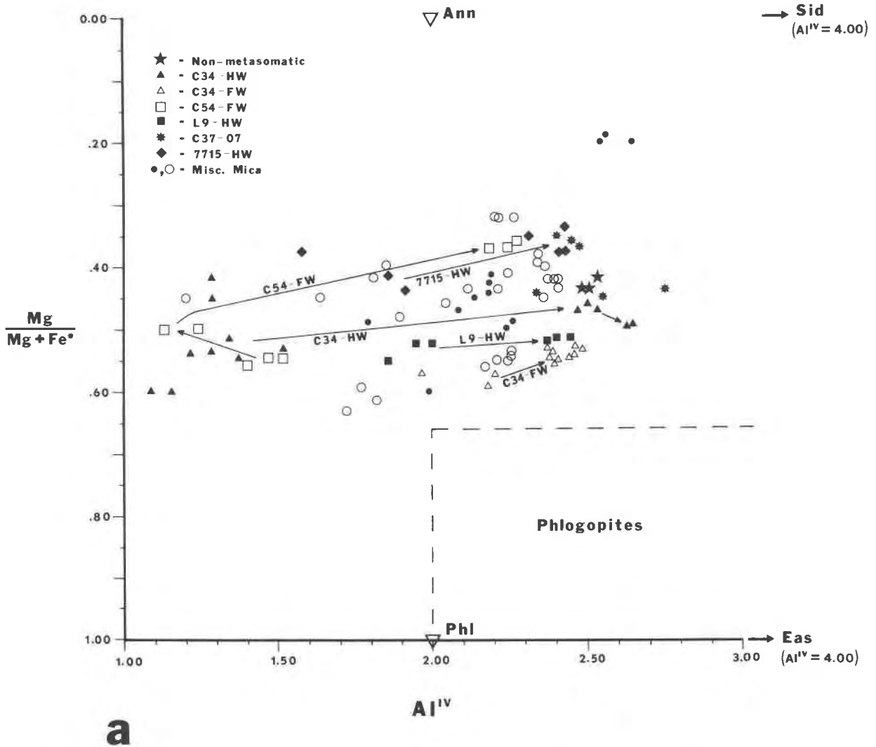
Fig. 5. (a) ^{IV}Al vs. Mg/(Mg + Fe_{total}) for exomorphic micas and non-metasomatic micas. (b) ^{IV}Al/Al_{total} vs. (Mg + Mn + Ti + Fe_{total})/6 for exomorphic micas and non-metasomatic micas. Arrows show the trends of micas from individual drill cores with increasing distance from the pegmatite contact. Ideal compositions of annite, siderophyllite, phlogopite, eastonite, polyolithionite, trilithionite, and taeniolite are after Bailey (1984). Ideal composition of zinnwaldite is after Hawthorne and Cerný (1982).
