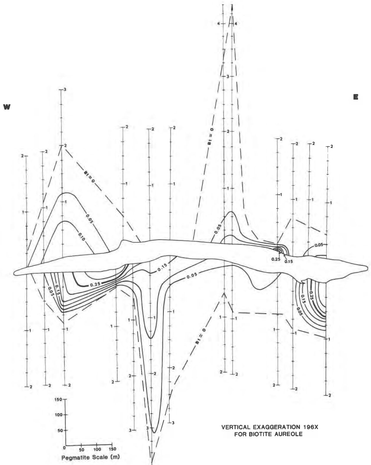
Fig. 7. Contour of the variation in cations of Cs per formula unit of exomorphic biotite from around the Tanco pegmatite.
