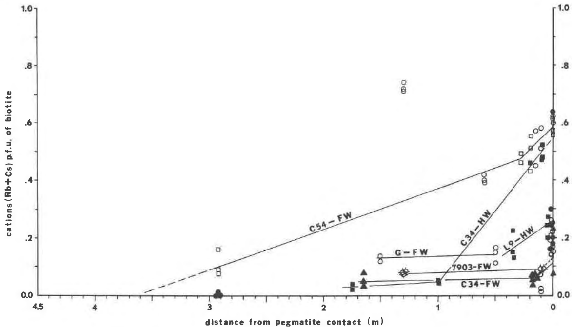
Fig. 9. Cation total (Rb + Cs) per formula unit of exomorphitic biotite vs. distance from the Tanco pegmatite. Open symbols indicate footwall samples; closed symbols indicate hanging-wall samples.
