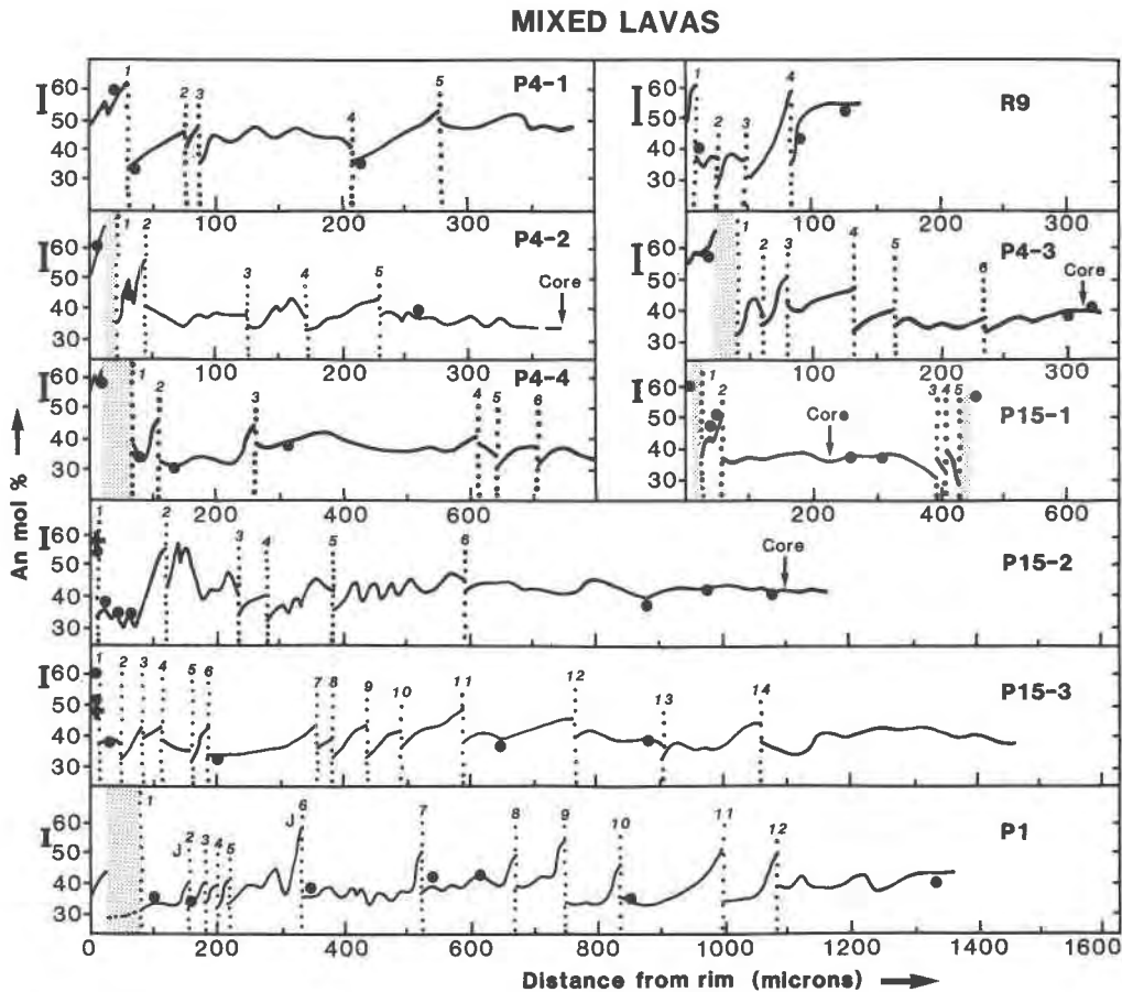
Fig. 9. Representative zoning profiles of plagioclase phenocrysts in mixed lavas (P1, P4, P15, and R9). Symbols are the same as in Fig. 7.
