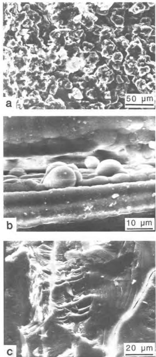
Fig. 1. Surface microstructures of opal speleothems under the SEM. (a) Colloidal aggregate (8416-12); coralloid from South Bald Rock Cave. (b) Colloform surface (8316-10); zeolite pseudomorph from Mt. Hamilton Cave. (c) Conchoidal fracture surface (8516-3); coralloid from Mt. Hamilton Cave.
