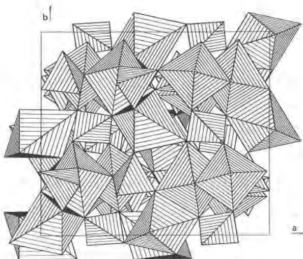
Fig. 2. Projection along c of the polyhedra arrangement in the grischunitite structure.
