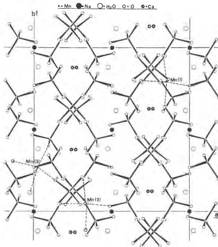
Fig. 1. Projection along c of the grischunitite structure.
