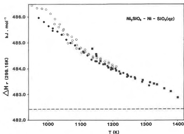
Fig. 6. Standard enthalpy, \Delta_r H_{m,298.15}^{\circ} , for the reaction 2\text{Ni} + \text{SiO}_{2(2qz)} + \text{O}_2 = \text{Ni}_2\text{SiO}_{4(\text{olivine})} calculated for each datum using the calorimetric data of Table 5. ■, run Ni-OL 1; ●, Ni-OL 2 (both vs. Ni + NiO); ○, Ni-OL 4 (vs. Fe + "FeO"). The dashed line is the result obtained using the heat-capacity data of Robie et al. (1984) together with the observed decomposition temperature of Ni 2 SiO 4 (1820 K).
