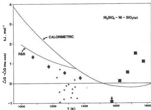
Fig. 7. Comparison showing the difference between various experimental determinations of the free energy of the reaction 2Ni + SiO_2 + O_2 = Ni_2SiO_4 and that of this work. The free energy of the reaction determined from the heat-capacity data of Robie et al. (1984) coupled with the observed decomposition temperature of Ni 2 SiO 4 (1820 K) is labeled "calorimetric." R&B: Rog and Borchardt (1984); ●, Levitskii et al. (1975); ◆, Taylor and Schmalzried (1964). For these three studies, the values for the Ni + NiO equilibrium found in this work were used to recalculate the results. ■, Campbell and Roeder (1968) (the datum at 1573 K, indicated by the arrow, actually plots at -2.36 kJ·mol -1 ).
