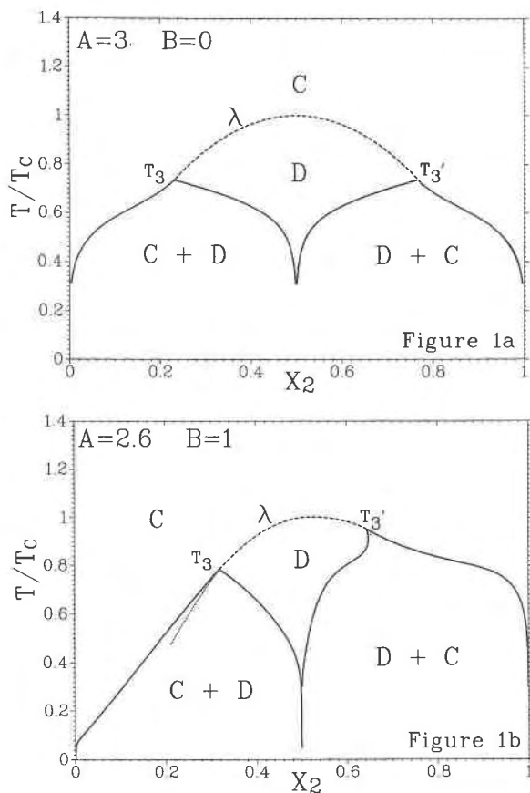
Fig. 1. (a) The symmetrical composition vs. temperature diagram ( \epsilon_{ier} = -1 , \epsilon_{ira} = 3 ); C = calcite-structure phase, D = dolomite-structure phase. (b) asymmetrical diagram, calculated with \epsilon_{ijk} , A = 2.6 , and B = 1 .
