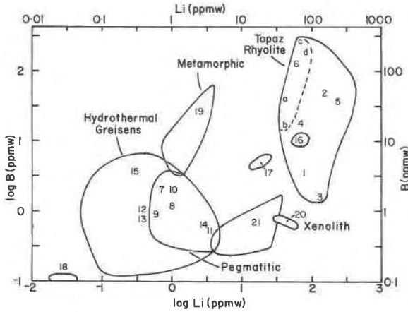
Fig. 1. Variation of the log of Li content vs. log of B content in topaz in parts per million by weight (ppmw). Numbers are placed at the mean composition for each locality, and solid lines encompass all analyses from an association. The areas labeled 16, 17, and 18 represent an ongonite and a topazite from Arizona and a topazite from N.S.W. Australia, respectively. Sample 21 is from the Henderson porphyry molybdenite deposit. See Table 1 for other localities.
