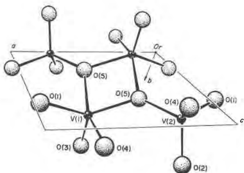
Fig. 5. One unit of the melanovanadate layer in oblique view.
