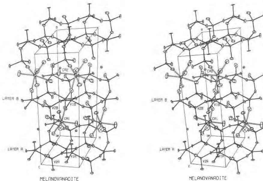
Fig. 4. Stereoscopic edge view of layer structure of melanovanadite, showing how a Ca ion is coordinated to one terminal oxygen atom of each adjacent layer, and 5 H 2 O molecules. The unlinked site labeled Ca2 is 10% occupied. Atoms are shown as 50% probability thermal ellipsoids.
