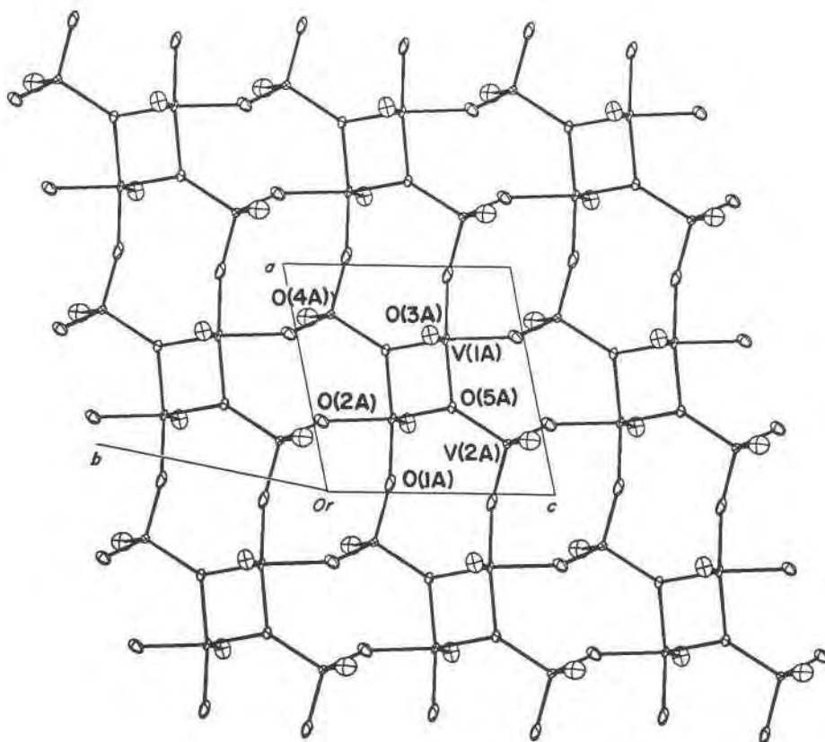
Fig. 3. The vanadate layer A of melanovanadite ( \nu \approx 0 ) viewed normal to the layer, showing 50% probability ellipsoids.
