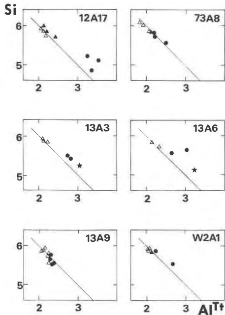
Fig. 3. The distribution of Si and Al Tt (Tt = total) in phlogopites: solid circles (core) and solid triangles (rim), micas associated with aluminous spinels; open triangles, authigenic micas; solid stars, micas found within clusters.
