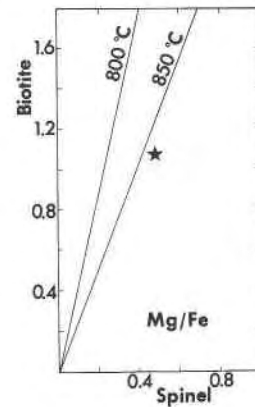
Fig. 5. Distribution of Mg/Fe total in spinels and coexisting biotites. Lines of best fit for experimental data at 800°C and 850°C from Brearley (1987). Solid star, specimen 12A17.
