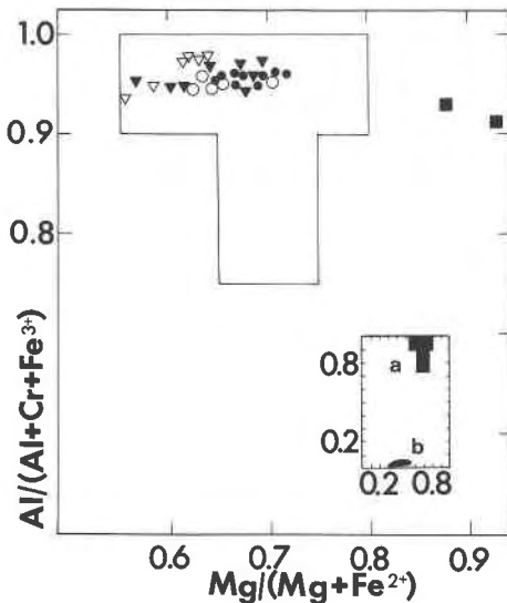
Fig. 2. Composition of aluminous spinels included in phlogopite in terms of \text{Al}/(\text{Al} + \text{Cr} + \text{Fe}^{3+}) vs. \text{Mg}/(\text{Mg} + \text{Fe}^{2+}) . Data from this study: open triangles, 12A17; solid triangles, 73A8; open circles, 13A3; solid circles, 13A9; solid squares, W2A1. Insert graph: data from Jaques and Foley (1985): (a) aluminous spinels included in leucite; (b) coexisting groundmass Cr-rich spinels.
