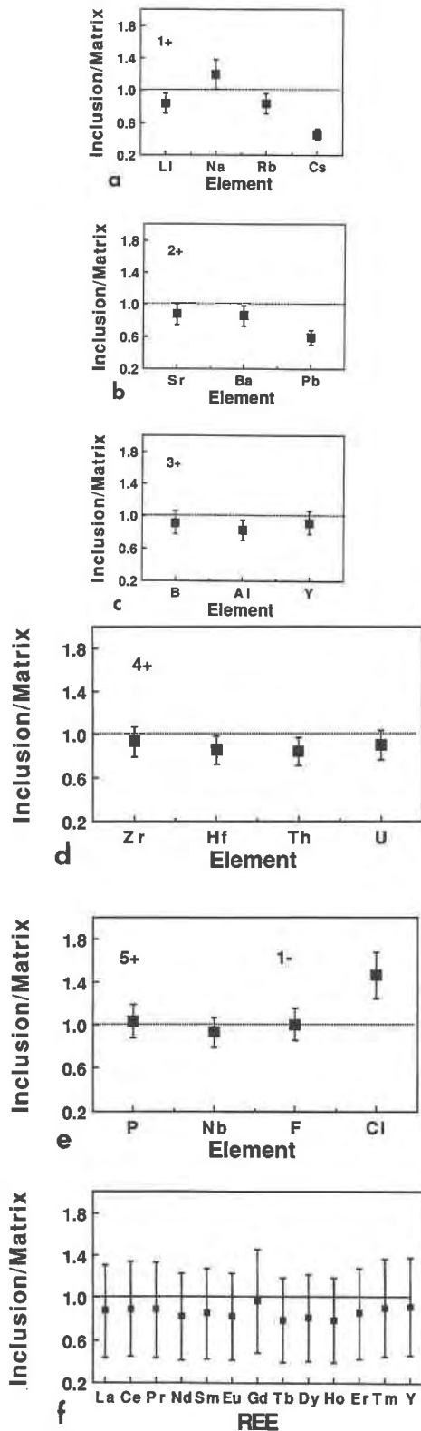
Fig. 2. Inclusion/matrix ratios for trace and major elements from a large (100- \mu m) inclusion in quartz compared to nearby matrix glass. Inclusion chemistry recalculated on an anhydrous basis for comparison with matrix. Errors for most trace elements are \pm 15\% relative on the basis of reproducibility of multiple analyses. Errors for rare-earth elements \leq 50\% .
