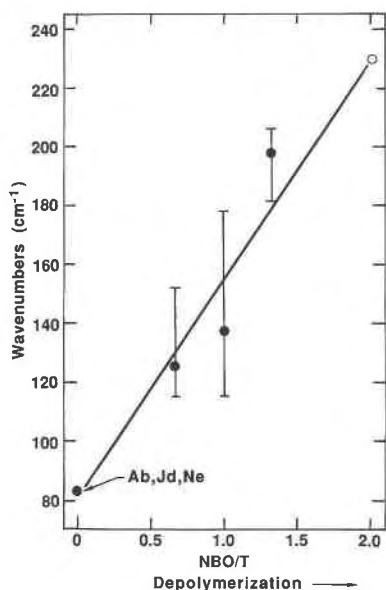
Fig. 5. Position of the low-frequency mode as a function of depolymerization. Open circle is a value from Exarhos and Risen (1972). Error bars indicate uncertainty in the position of the broader peaks in the sodium silicate glass spectra. Error in the peak positions in the mineral-glass spectra is approximately the size of the closed circle.
