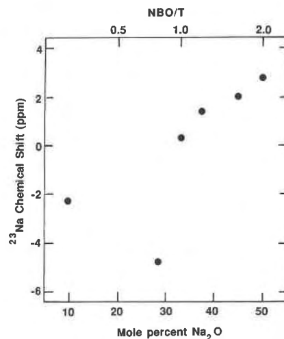
Fig. 6. ^{23}\text{Na} chemical shift for \text{Na}_2\text{O}-\text{SiO}_2 glasses as a function of Na content. Data from Dupree et al. (1984).
