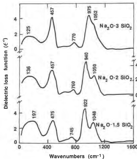
Fig. 4. Dielectric loss functions ( \epsilon'' ) of glasses along the \text{Na}_2\text{O}-\text{SiO}_2 join. The values of \epsilon'' for \text{Na}_2\text{O}\cdot 3\text{SiO}_2 and \text{Na}_2\text{O}\cdot 1.5\text{SiO}_2 are shown on the left, and those for \text{Na}_2\text{O}\cdot 2\text{SiO}_2 are on the right.
