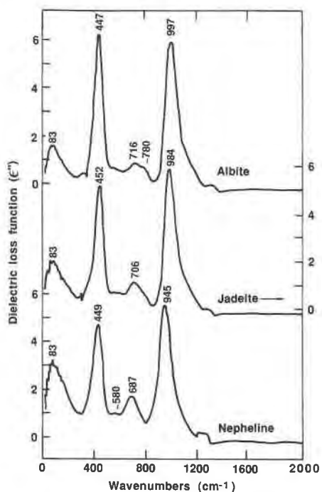
Fig. 2. Dielectric loss functions ( \epsilon'' ) of albite, jadeite, and nepheline glass. The abscissa is scaled as for Fig. 1.
