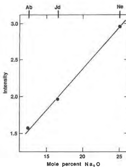
Fig. 3. Peak height of the low-frequency mode in \epsilon'' as a function of Na content.
