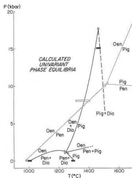
Fig. 2. P - T projections of calculated univariant reactions involving protoenstatite, orthoenstatite, pigeonite, and diopside (from Carlson and Lindsley, 1988), illustrating calculated stability of protoenstatite + pigeonite in place of orthoenstatite near 1400 °C and 1 bar. Bold lines depict ternary equilibria in CaO - MgO - SiO_2 ; lighter lines depict binary equilibria among the Ca-free end members. Equilibria are computed from a thermodynamic model constrained by experimental data indicated by rectangles and by additional data extending to 1600 °C and 60 kbar. Calculated supersolidus equilibria (metastable relative to silicate melts) at T > \sim 1400 °C and P < \sim 5 kbar are omitted.
