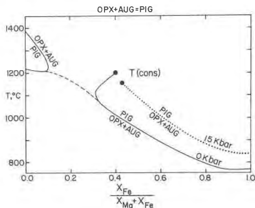
Fig. 3. Stability relations of Pig predicted by a quadrilateral solution model that incorporates the Carlson and Lindsley (1988) model for Di-En. Melting relations are not shown. The predicted gap in the stability of Pig at 0.10 < \text{Fe}/(\text{Fe} + \text{Mg}) < 0.30 is incompatible with a variety of experimental data and natural occurrences for which the minimum stability of Pig is indicated by the dashed line. T(\text{cons}) indicates the intersection of the calculated \text{Pig} = \text{Opx} + \text{Aug} reaction with the \text{Pig} - \text{Aug} consolute temperature.
