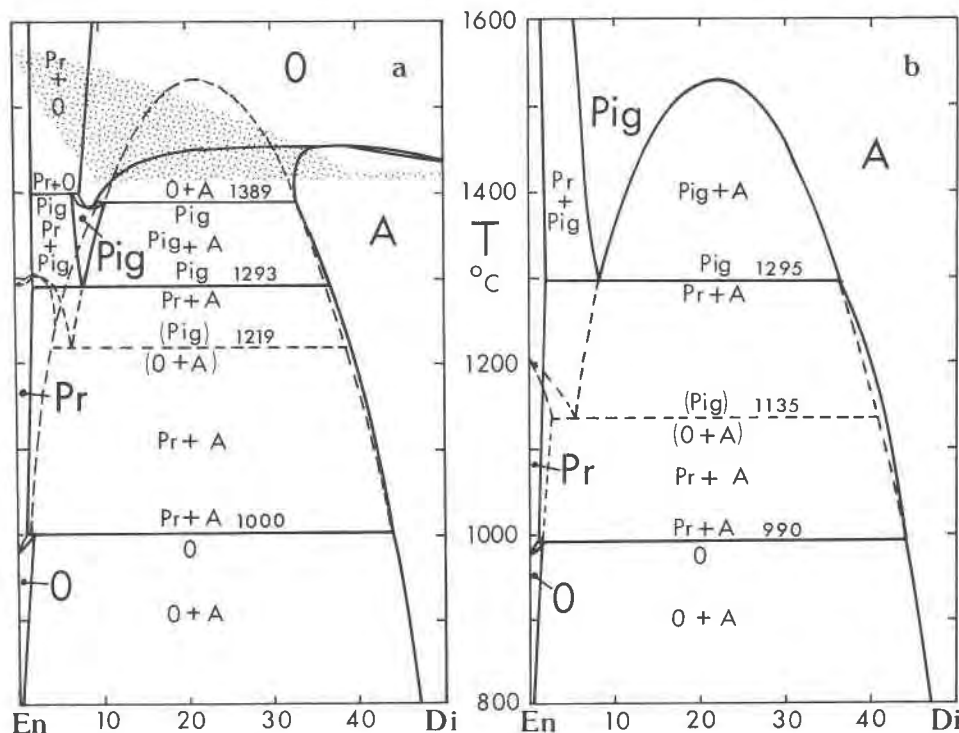
Fig. 2. Phase relations calculated at 1 atm from the Carlson and Lindsley (1988) model (a) and the revised solution model presented in this work (b). The melting interval is indicated by the stippled area in (a). Abbreviations as in Fig. 1. The Carlson and Lindsley model correctly predicts the re-appearance of orthopyroxene at near-solidus temperatures (Longhi and Boudreau, 1980; Carlson, 1988), but the relative compositions of O
