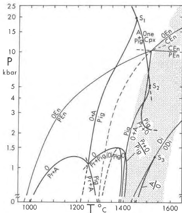
Fig. 1. P - T projection for the system Mg_2Si_2O_6 - CaMgSi_2O_6 based on the Carlson and Lindsley (1988) model. This is an extension of Fig. 2 of Carlson and Lindsley. Melting relations are omitted, but the melting interval is approximated by the stippled area. Note log P scale. End-member phases are indicated as OEn, orthoenstatite; CEn, clinoenstatite; PEn, protoenstatite; Di, (clino)diopside; ODi, "orthodiopside." Solid solutions are abbreviated as O, orthopyroxene, some highly calcic; Pig, low-Ca clinopyroxene; A, high-Ca clinopyroxene; Pr, protopyroxene. Abbreviations in parentheses label metastable curves. S_1 , S_2 , and S_3 are singular points.
