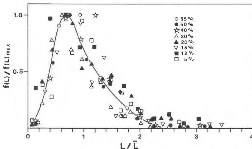
Fig. 6. Length of illite/smectite grains normalized to the mode as a function of percent expandable layers. The curve has been smoothed.
