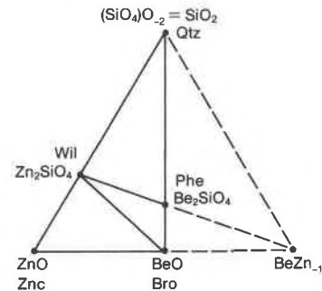
Fig. 3. Presumed low-pressure mineral compatibilities in the reciprocal system /Zn,Be//O,SiO_2/ , which could also be described as the system ZnO-BeO-SiO_2 . The figure shows that Zn has a greater affinity for silica than Be does.
