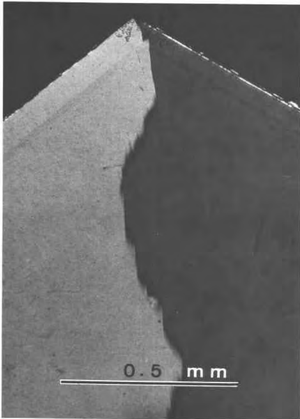
Fig. 3. Cross-polarized photomicrograph of \{10\bar{1}\} sectors in the (010) thin section. The crystal has two \{10\bar{1}\} faces and two corresponding \{10\bar{1}\} sectors, which are related by the (100) twinning with comblike composition plane. The c axis is vertical. Epistilbite from Fossarfell, Iceland.
