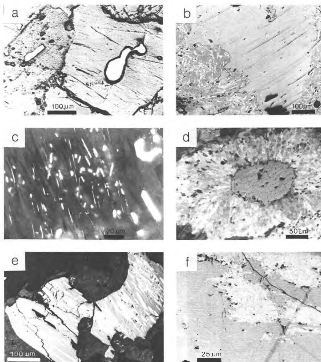
Fig. 3. Ilmenite features: (a) Anhedrally subrounded ilmenite inclusions in biotite, typical mode of occurrence of ilmenite in S-type granites; KB-45, PRL, OI. (b) Biotite surrounded by abundant ilmenite laths in quartz and feldspar; the biotite is embayed and corroded; S-type, MB-15, PRL. (c) Amphibole containing fine-grained ilmenite laths in its core; the ilmenites are oriented parallel to the c axis of the amphibole and may be due to exsolution; I-type, MG-23, PRL, OI. (d) Corroded ilmenite grain with a radiating rim of titanite, possibly formed by inward replacement of ilmenite rather than as an outward overgrowth rim; I-type, CB-61, partly XRL, OI. (e) Ilmenite grains containing hematite exsolution lamellae included in a large grain of titanite; I-type, MG-23, PRL, OI. (f) Part of a large ilmenite grain containing hematite exsolution lamellae; two twin planes cut across the grain. The ilmenite contains patches of alteration to hematite and rutile; I-type, KB-28, PRL. For key to abbreviations, see Fig. 2.
