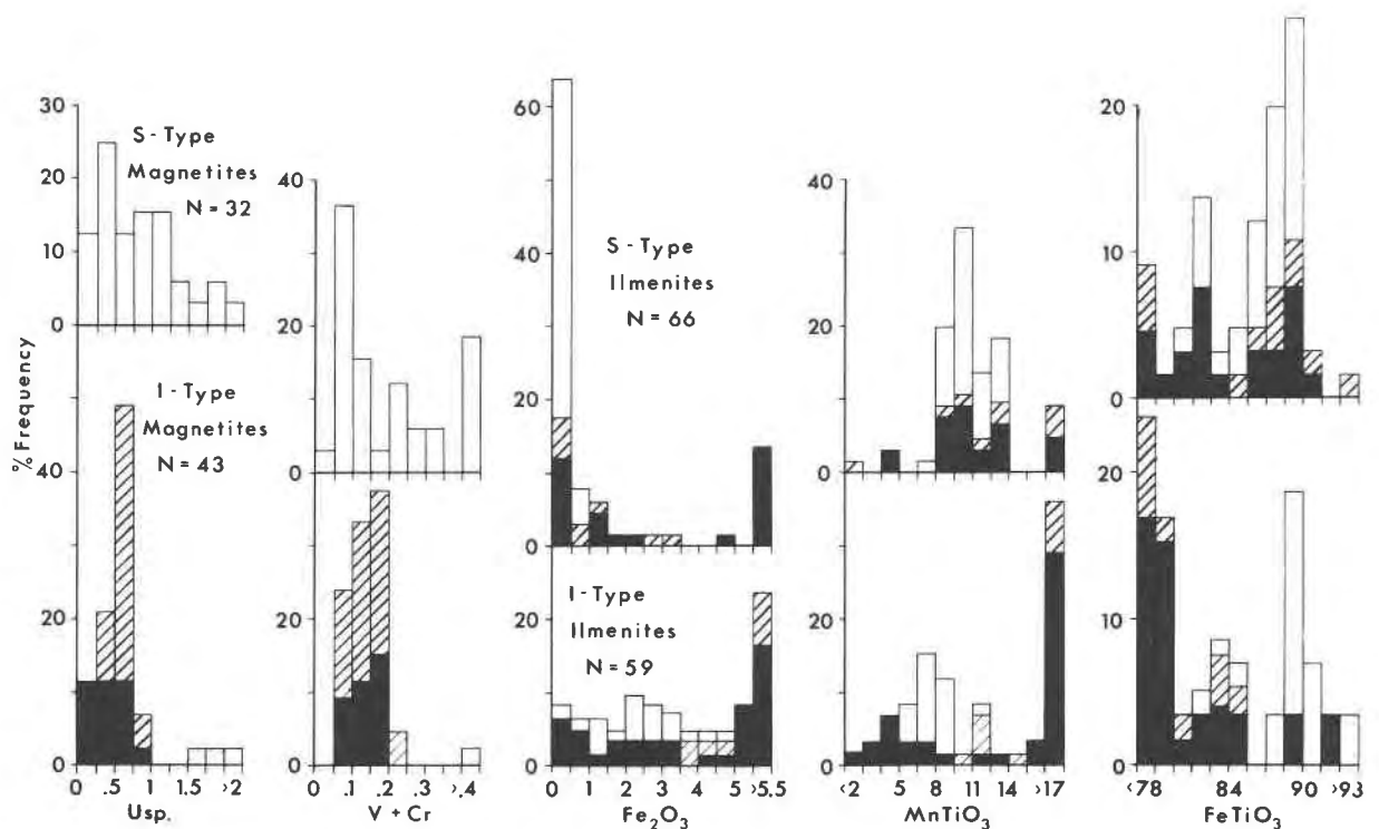
Fig. 9. Histograms of some features of Fe-Ti oxide mineral chemistry. S-type granites are shown in the top group of histograms; for ilmenites, shaded portions are from magnetite-bearing S-type granites, cross-hatched portions are from Dalgety and Shannons Flat samples in which magnetite has not been identified, and unpatterned portions are from magnetite-free S-type granites. I-type granites are shown in the bottom group of histograms; shaded portions are from the Moruya suite, cross-hatched portions are from Jindabyne samples, and unpatterned portions are from the Finister suite. N = number of grains.
