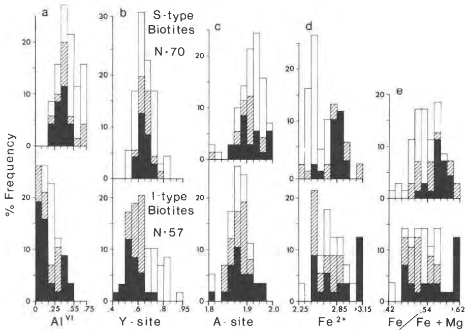
Fig. 10. Histograms of some features of biotite chemistry. S-type granites are shown in the top grouping of histograms; shading types for different suites as in Fig. 9. N = number of grains.
