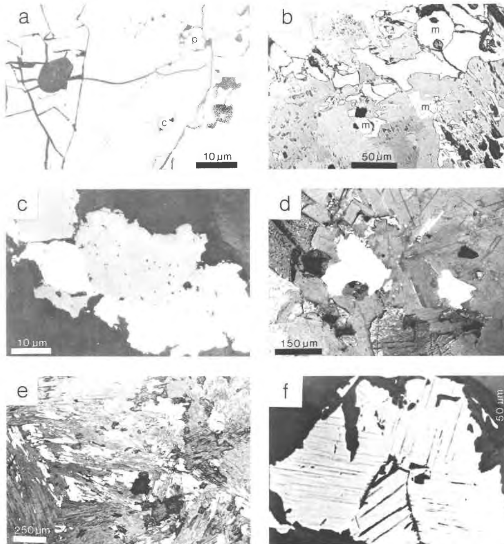
Fig. 4. Sulfide features: (a) A composite magnetite-ilmenite grain; the ilmenite contains both pyrite (p) and chalcopyrite (c) inclusions; I-type, BB-10, PRL, OI. (b) Pyrite rimming magnetite (m) and replacing amphibole in a veining dendritelike form; I-type, AB-17, PRL. (c) Composite ilmenite-pyrite-chalcopyrite aggregate within a biotite aggregate. Chalcopyrite occurs as an interstitial filling between pyrite and ilmenite grains; the sulfide does not appear to replace the ilmenite; S-type, BB-83, PRL, OI. (d) Pyrite grains in a biotite aggregate; between some biotite grains there is ilmenite that has exsolved from biotite; BB-36, PRL. (e) Aggregate of sillimanite and partly interstitial pyrrhotite in a S-type xenolith; BB-146, PRL. (f) Aggregate of pyrrhotite grains with alteration along cleavage partings; S-type, CB-35, PRL. For key to abbreviations, see Fig. 2.
