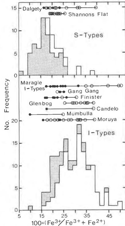
Fig. 8. Histograms of whole-rock 100\text{Fe}^{3+}/(\text{Fe}^{3+} + \text{Fe}^{2+}) for studied I- and S-type granite samples. In the upper histogram for S-type granites, the shaded area is for samples lacking magnetite and the unshaded areas are for magnetite-bearing samples. Above the histogram are plotted samples from the two magnetite-bearing S-type suites (Dalgety and Shannons Flat); open and closed circles represent samples that contain and lack magnetite, respectively. In the lower histogram for I-type granites, the shaded and unshaded areas represent samples containing less than and greater than 10% magnetite, respectively. Plotted above the histogram are suites with low magnetite contents; filled and open circles correspond to samples containing less than and greater than 10% magnetite, respectively. Magnetite-bearing S-type granites are more oxidized, and magnetite-poor I-type granites are more reduced, than the mean of their respective groups.
