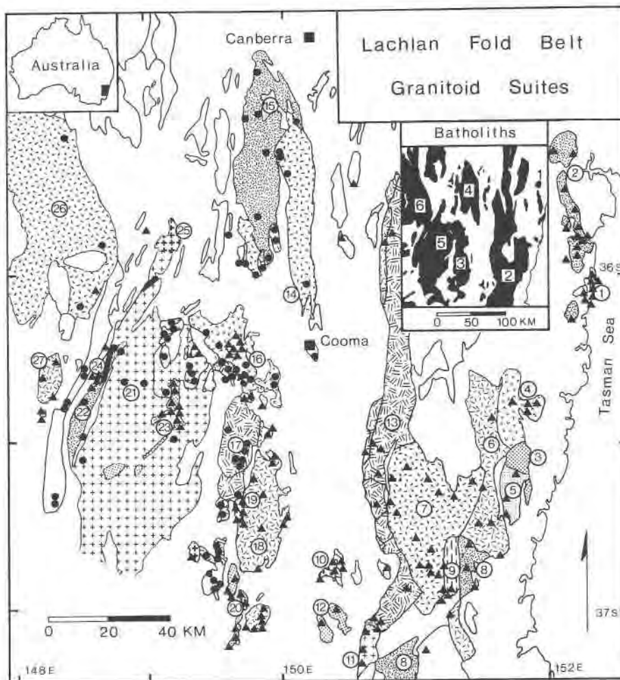
Fig. 1. Location of different I- and S-type granitoid suites and opaque mineral samples (I-type = filled triangles; S-type = filled circles) in part of the Lachlan fold belt. The main batholiths are numbered in the insert on the upper right: (1) Moruya, (2) Bega, (3) Berridale, (4) Murrumbidgee, (5) Kosciusko, (6) Maragle. The following main suites (designated I- or S-type in parentheses) are shown with different patterns and numbered in circles: (1) Bingie Bingie (I), (2) Moruya (I), (3) Mumbulla (I), (4) Cobargo (I), (5) Brogo (I), (6) Kameruka (I), (7) Bemboka (I), (8) Candelo (I), (9) Why Worry (I), (10) Kelvin (I), (11) Tonghi (I), (12) Flat Rock (I), (13) Glenbog (I), (14) Clear Range (I), (15) Shannons Flat (S), (16) Cootralantra (S), (17) Dalgety (S), (18) Buckleys Lake (I), (19) Finister (I), (20) Currowong (I), (21) Bullenbulong (S), (22) The Ghost (S), (23) Jindabyne (I), (24) Gang Gang (I), (25) Boggy Plains (I), (26) Green Hills (S), (27) Khancoban (I). (Based on sources given in Table 1 and unpublished data of B. W. Chappell.)
