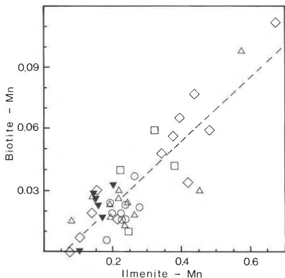
Fig. 13. Plot of Mn content of biotite vs. Mn content of ilmenite with calculated regression line; each point represents a rock sample. Suite symbols: ( \diamond ) Moruya; ( \square ) Jindabyne; ( \blacktriangledown ) Finister; ( \triangle ) magnetite-bearing S-types; ( \circ ) magnetite-free S-types.
