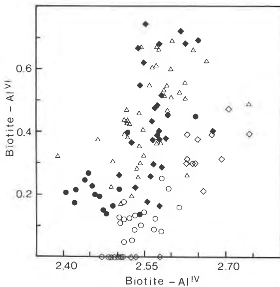
Fig. 11. Plot of {}^{\text{IV}}\text{Al} vs. {}^{\text{VI}}\text{Al} for biotites coexisting with (○) amphibole, (●) amphibole in Finister suite, (◇) biotite alone in I-types, (△) biotite alone in S-types, (◆) muscovite in S-types.
