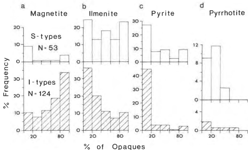
Fig. 6. Histograms of the visually estimated percentages (i.e., not point counted) of magnetite, ilmenite, pyrite, and pyrrhotite in S-type (top histograms) and I-type (lower histograms) granites and xenoliths. Only a portion of the samples plotted in Fig. 5 was studied.
