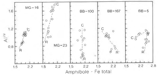
Fig. 12. Zoning of IV Al vs. total Fe as Fe 2+ in amphibole from the Moruya (MG-16), Bingie Bingie (MG-23), and Finister (BB-100, 167, 5) suites. Point analysis (O), grain core (C) and rim (R) positions, and visually estimated trends for the data (dashed lines) are plotted.
