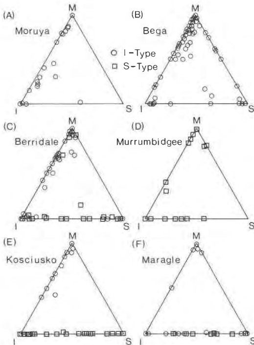
Fig. 7. Triangular diagrams for opaque mineral assemblages in I- and S-type granites of different batholiths of the Lachlan fold belt; ilmenite (I), magnetite (M), and total sulfides (S).
