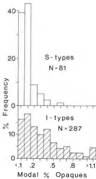
Fig. 5. Histograms of the modal percentage of opaque minerals in S- and I-type granites of the Lachlan fold belt. Based on all available unpublished modal data of B. W. Chappell.
